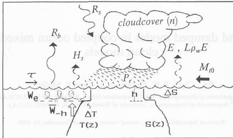
Fig. 1. Main physical processes in the two adjacent boundary layers.
