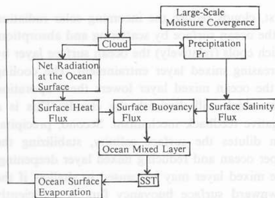
Fig. 2. Feedback paths between OPBL and clouds.
