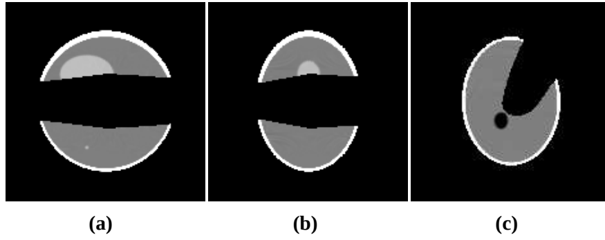
Figure 13: Images within slices at x = 0 cm (a), y = 0 cm (b), and z = -2.5 cm (c) reconstructed from noiseless data by use of the chord-based algorithm on both one-turn and two-turn chords.
