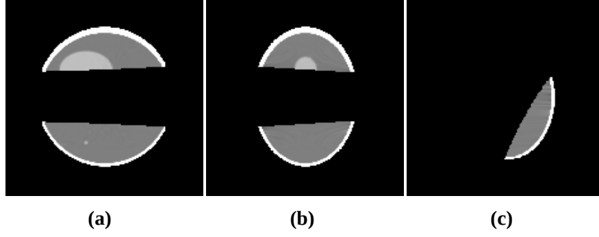
Figure 12: Images within slices at x = 0 cm (a), y = 0 cm (b), and z = -2.5 cm (c) reconstructed from noiseless data by use of the chord-based algorithm on one-turn chords. The display window used in this paper is [1.0, 1.04] .
