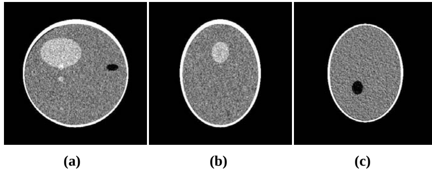
Figure 16: Images within slices at x = 0 cm (a), y = 0 cm (b), and z = -2.5 cm (c) reconstructed from the noisy data by use of the proposed FBP algorithm.
