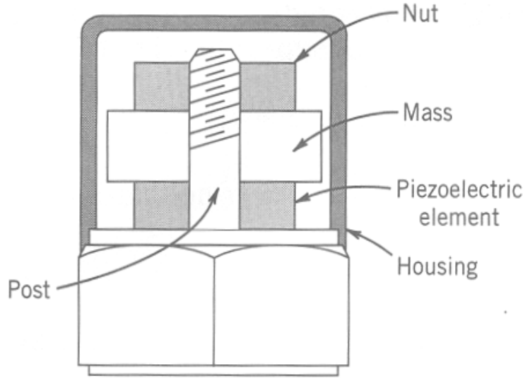
Figure 2.13: Piezoelectric Accelerometer [45]
