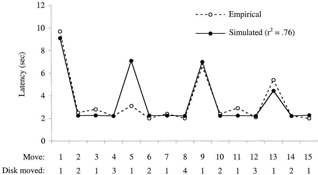
Fig. 7. Move latencies for four-disk problems. Empirical values are from Table 1. Simulated values are from the goal-activation model lesioned to disable goal retrieval.
