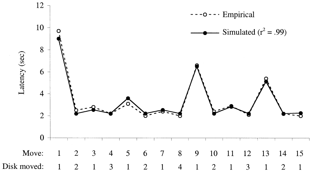
Fig. 5. Move latencies for four-disk problems. Empirical values are from Table 1. Simulated values are from the goal-activation model.
