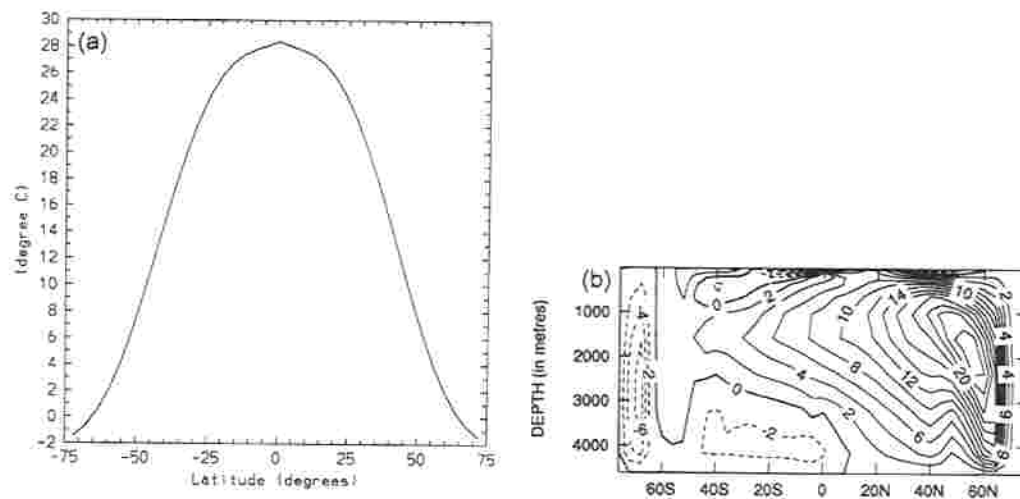
Figure 1. (a) Surface relaxation temperature ( ^{\circ}\text{C} ), and (b) overturning stream function ( \text{Sv} ) for R15o, that is, under a restoration with a restoring time of 15 days, and initiated from a resting ocean.
