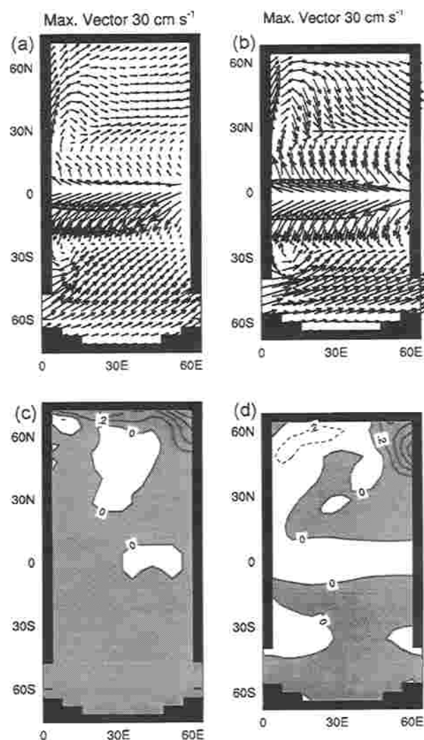
Figure 8. (a) and (b) Steady surface flow vectors of R30o and R45oShB respectively. From the steady state of these two runs, runs R30p and R45ShBp are initiated. In each run a heat anomaly is imposed over the three northern-most grid-points along the eastern boundary, and lasts for six months; (c) and (d) distribution of SST anomaly ( ^{\circ}\text{C} ) 5 years after the anomaly is removed for R30p and R45ShBp respectively.
