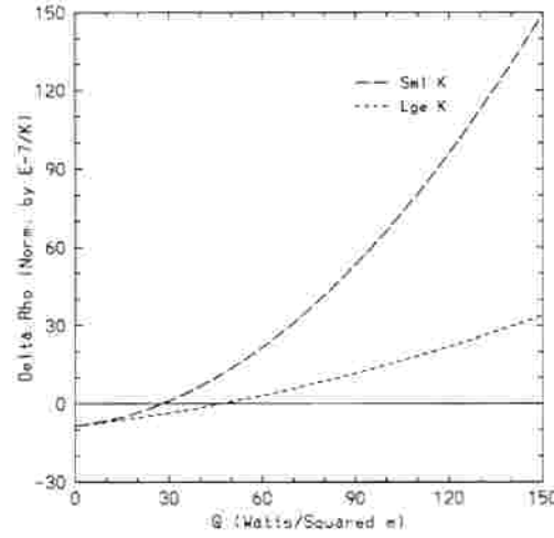
Figure A.1. Dependence of density difference ( \rho_1 - \rho_2 ) ( \text{kg m}^{-3} ) upon subsurface heating in a two-layered thermal flip-flop model. When the subsurface heating Q ranges from 26 to 45 \text{ W m}^{-2} , the flip-flop model is in an oscillatory regime. In this regime, once convection occurs (large K ) the water column becomes stable ( \delta\rho < 0 ), whereas once convection stops (small K ), the water column becomes unstable ( \delta\rho > 0 ).
