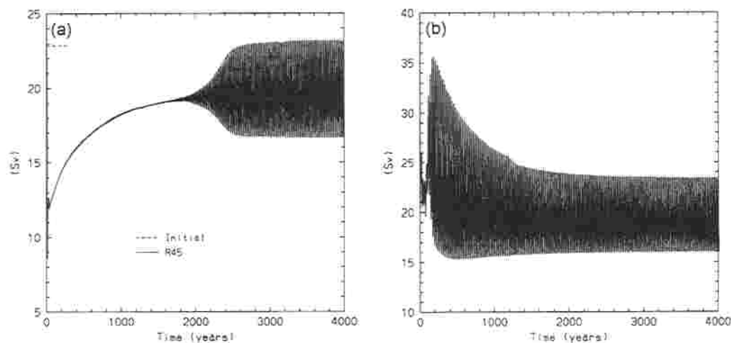
Figure 2. (a) Time series of the overturning (Sv) for run R45, that is, initiated from the steady state of R150 and under a restoration with a restoring time of 45 days. The overturning is sampled at a location ( 60^{\circ}\text{N} , 2350 m) near the place where the overturning of the steady state of R150 is a maximum. (b) Time series of the overturning (Sv) for run R450, that is, under a restoration with a restoring time of 45 days but initiated from a resting ocean.
