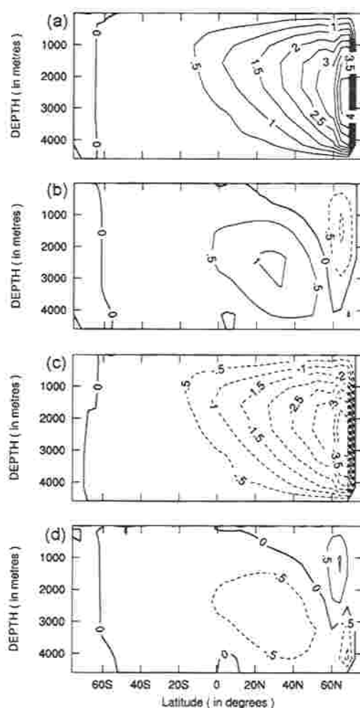
Figure 6. Anomalies of overturning ( S_v ) from a mean circulation for R4S at about a quarter period interval: (a) at year 3550; (b) at year 3554; (c) at year 3560; (d) at year 3569. Panels (a) and (d) show the anomalies when the overturning is at a maximum and a minimum respectively.
