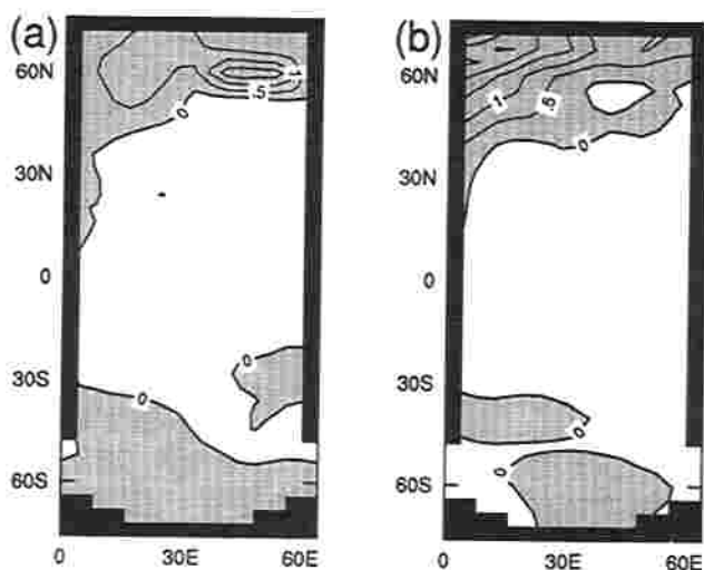
Figure 6. Sea surface temperature differences: (a) between the state at year 1112.5 (State I) and that at year 3337.5 (State II) (both when \alpha(t) = 0.5 ); (b) between the warm and cold phases of a typical oscillation.
