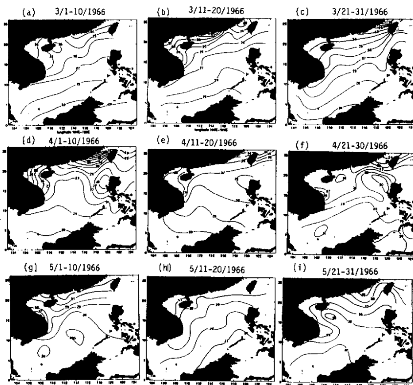
Fig. 4. Temporally varying sea surface temperature of the South China Sea from 1 March to 31 May, 1966.
