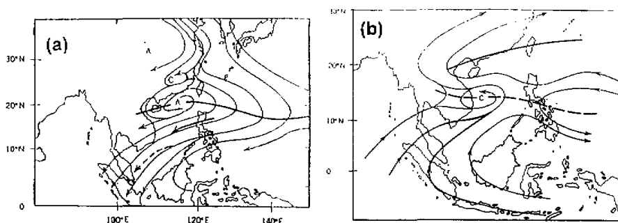
Fig. 5. Mean atmospheric surface streamline analysis for (a) winter, and (b) early spring (from Cheang, 1980).
