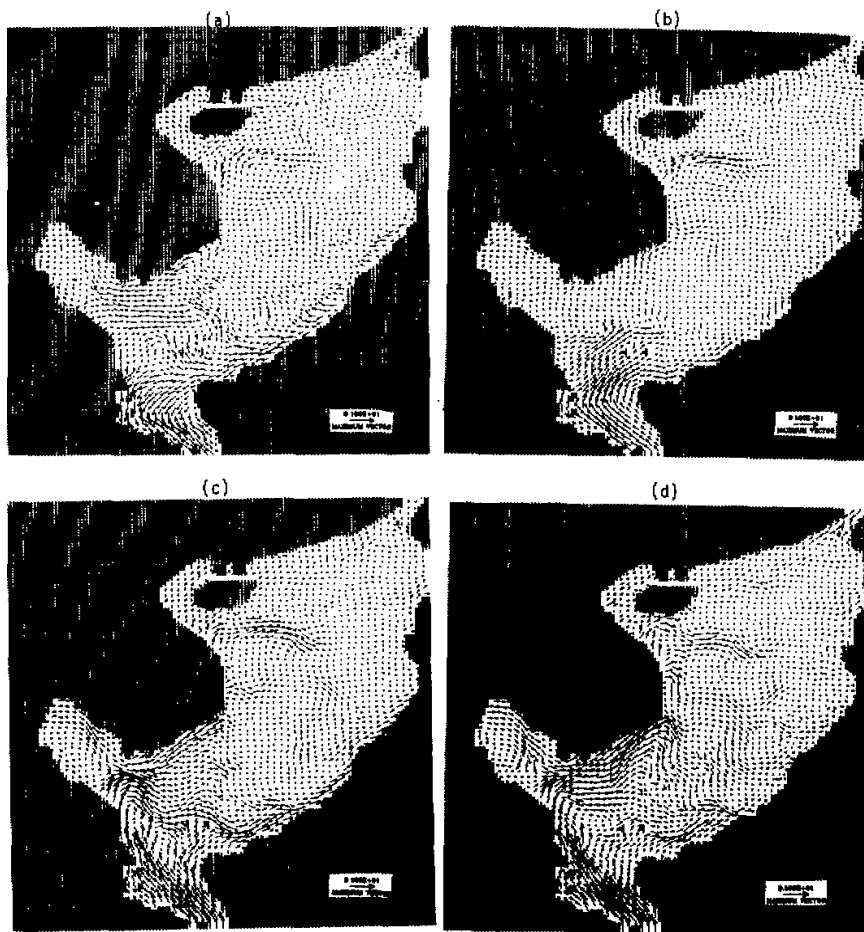
Fig. 8. Model simulated surface circulations for (a) 30 March, (b) 30 April, (c) 30 May, and (d) 30 June.
