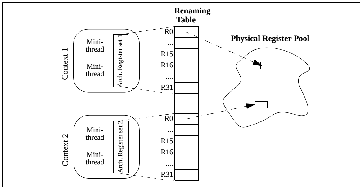
FIGURE 5.1: Register sharing among mini-threads on an \text{mtSMT}_{2,2} . There are two hardware contexts, each supporting two mini-threads that share architectural registers within the context.
