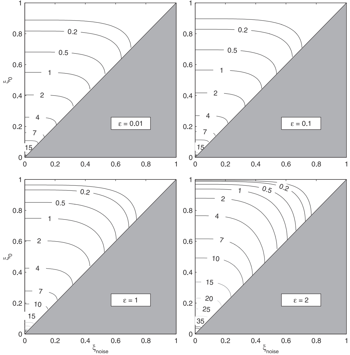
Figure 3. Contour plots of \tau_2(\bar{\xi}_0, \bar{\xi}_{\text{noise}}, \varepsilon) versus \bar{\xi}_0, \bar{\xi}_{\text{noise}} for four different values of \varepsilon (0.01, 0.1, 1, and 2) using the Nicolis [1992] model with stochastic forcing q^2 = 0.2 . The contour plot covers the half domain due to \bar{\xi}_0 \geq \bar{\xi}_{\text{noise}} .
