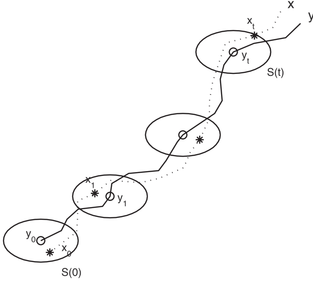
Figure 1. Phase space trajectories of model prediction y (solid curve) and reality x (dotted curve) and error ellipsoid S_e(t) centered at y . The positions of reality and prediction trajectories at time instances are denoted by asterisks and open circles, respectively. A valid prediction is represented by a time period (t - t_0) at which the
