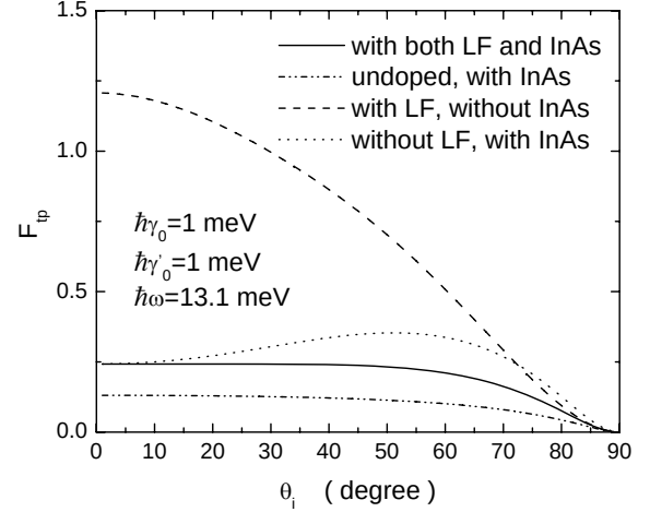
Fig. 11. Calculated F_{tp} for the p polarization as a function of \theta_i with \hbar\omega = \hbar\Omega_{3D}^{pl} = 13.1 \text{ meV} , \hbar\gamma_0 = 1 \text{ meV} , and \hbar\gamma'_0 = 1 \text{ meV} . The results of F_{tp} are compared for four different cases: (1) including both a longitudinal field and an InAs conducting sheet (solid curve); (2) with an undoped GaAs bulk ( n_{3D} = 0 ) and with an InAs conducting sheet (dash-dot-dotted curve); (3) without an InAs conducting sheet but with a longitudinal field (dashed curve); (4) without a longitudinal field but with an InAs conducting sheet (dotted curve).
