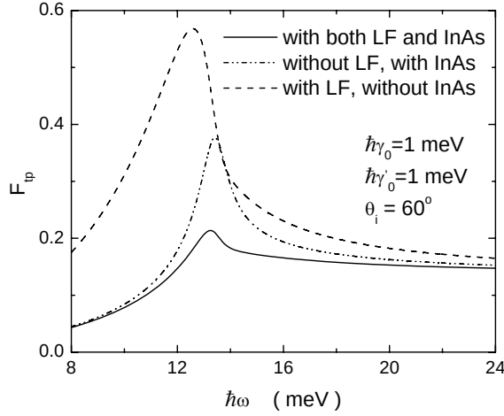
Fig. 10. Calculated F_{tp} for the p polarization as a function of the incident photon energy \hbar\omega with \theta_i = 60^\circ , \hbar\gamma_0 = 1 \text{ meV} , and \hbar\gamma'_0 = 1 \text{ meV} . The results of F_{tp} are compared for three different cases: (1) including both a longitudinal field (LF) and an InAs conducting sheet (solid curve); (2) without a longitudinal field but with an InAs conducting sheet (dash-dot-dotted curve); (3) without an InAs conducting sheet ( n_{2D} = 0 ) but with a longitudinal field (dashed curve).
