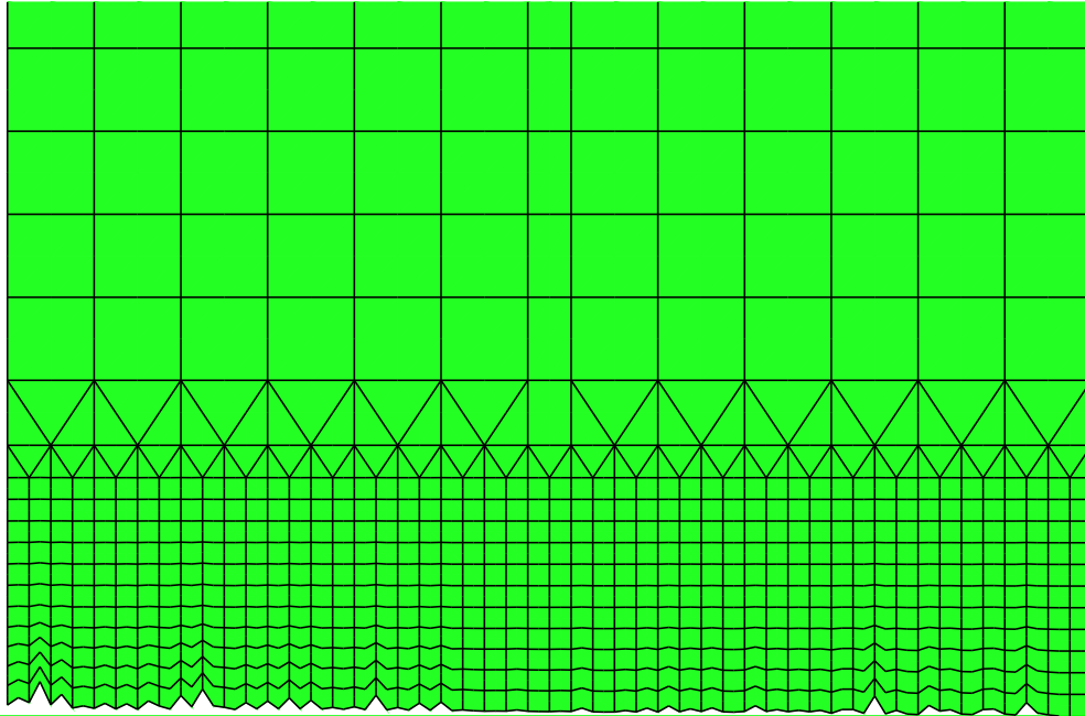
Figure 3.13: An example of an unrealistic wear profile that can cause an aborted analysis
