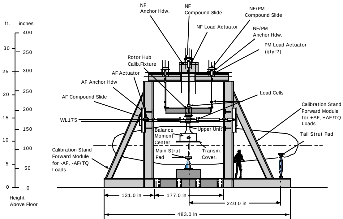
Figure 4: Schematic of the LRTA calibration rig
