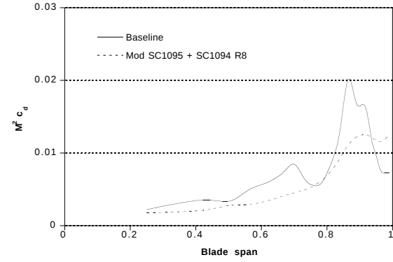
(b) M^2 c_d
