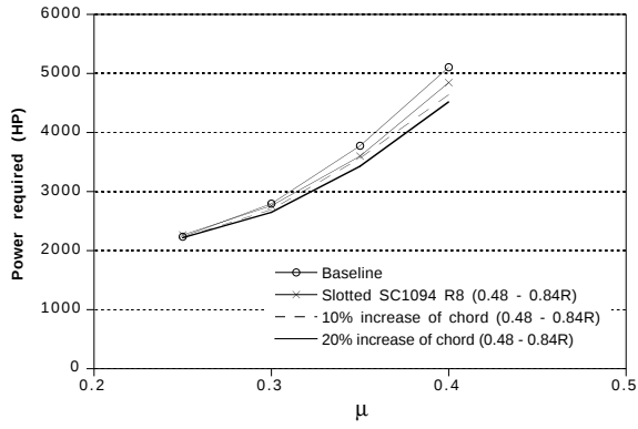
(c) Power required at C_T/\sigma = 0.12
