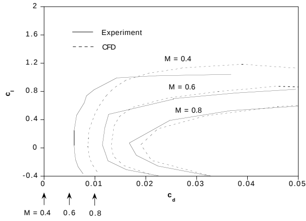
Fig. 4 Comparison of CFD results with experiment for RC(6)-08
