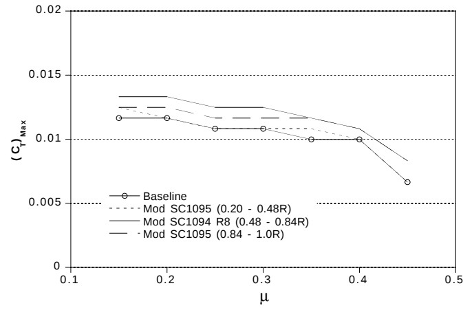
(b) Maximum thrust coefficient
