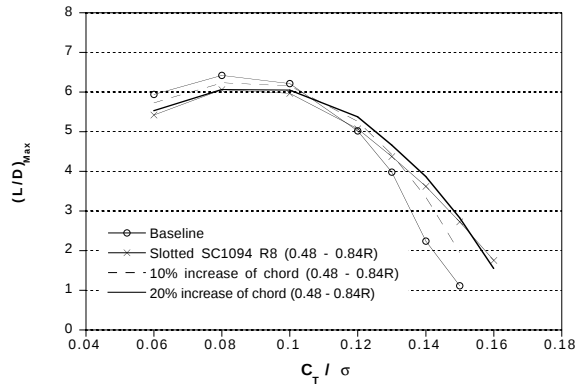
(a) Maximum lift-to-drag ratio
