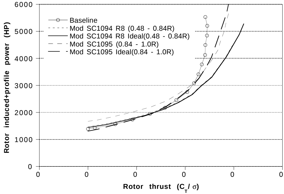
Fig. 15 Effect of ideal slotted airfoil on performance
