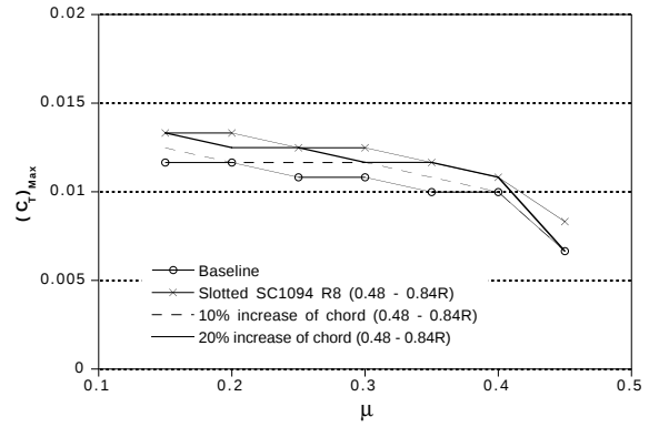
(b) Maximum thrust
