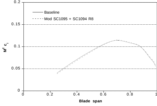
(a) M^2 c_l
