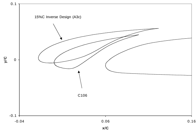
Fig. 1 C106 and A3c airfoil slat geometry [Ref. 4]
