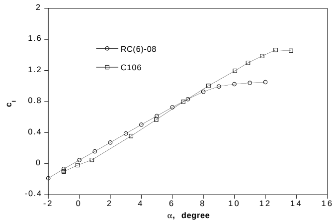
Fig. 2 Effect of slotted configuration on lift coefficients at M = 0.4
