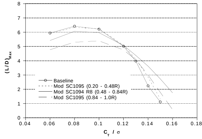
(a) Maximum lift-to-drag ratio
