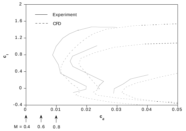
Fig. 5 Comparison of CFD results with experiment for C106
