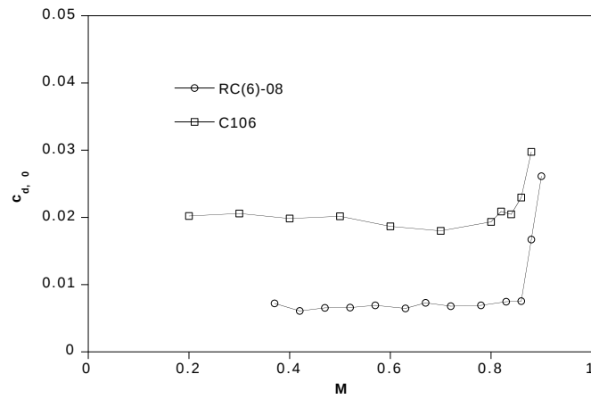
Fig. 3 Comparison of drag coefficients at zero lift angle of attack
