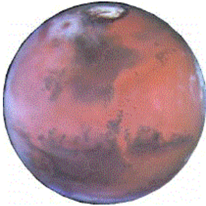
Fig.4 – Mars (Image from Hubble Space Telescope (HST))
