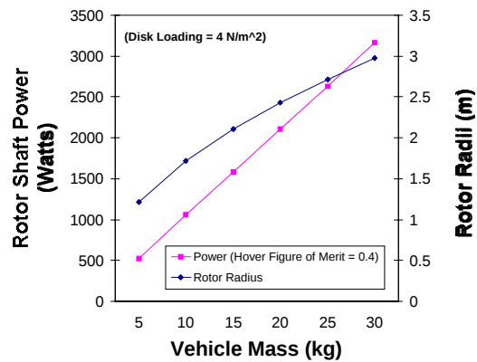
Fig. 5 – Martian Autonomous Rotorcraft: Large, Ultra-lightweight, Fragile-Looking...
