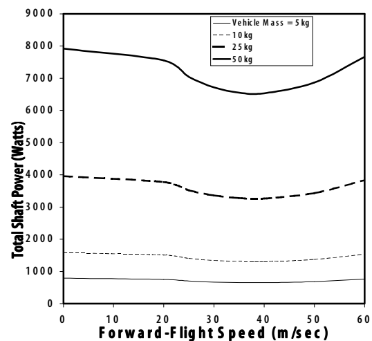
Fig. 8 – Mars Coaxial Helicopter Performance Estimates
