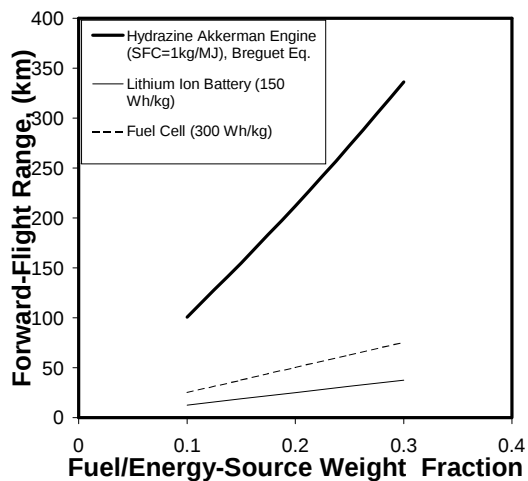
Fig. 9 – Mars Coaxial Helicopter Range Estimates
