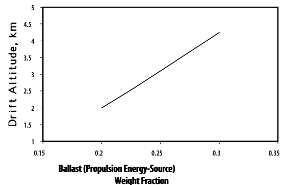
Fig. 17 -- ‘Drift’ Altitude of Unpowered Vehicle After Ballast Drop
