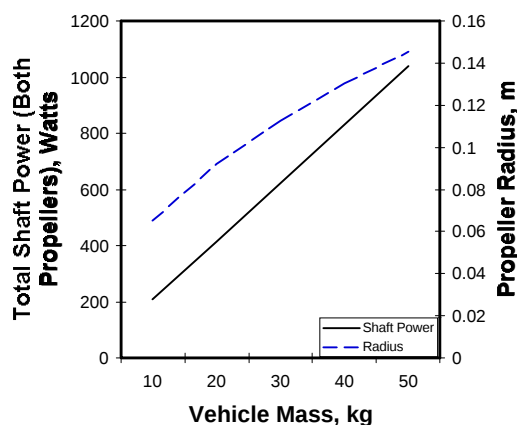
Fig 18 – Hybrid-Airship Tandem Propellers Hover Performance and Sizing Estimates
