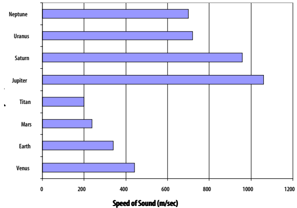
Fig. 2 – Estimates for the Speed of Sound
