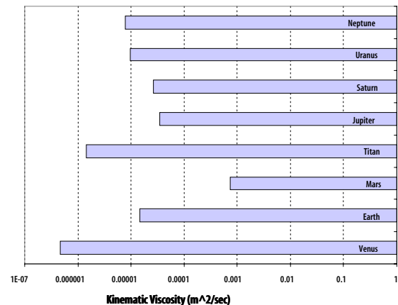
Fig. 3 – Estimates of Kinematic Viscosity
