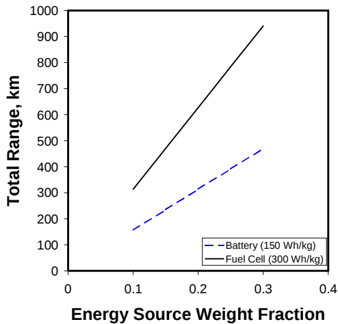
Fig. 13 – Range Estimates for a Twin Ducted Fan Titan VTOL
