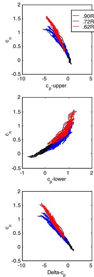
Fig. 4. c_n versus c_p plots for upper and lower blade pressure measurements for three radial locations
