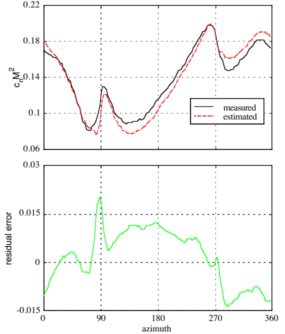
Fig. 14. Measured versus estimated airloads from regression model (input: c_{p,upper,3.5} M^2 , c_{p,lower,3.55} M^2 , \alpha , C_T/\sigma ) expressed as c_n M^2 and residual error as function of azimuth angle for database subset #7 ( \alpha=-10^\circ , C_T/\sigma=0.128 )
