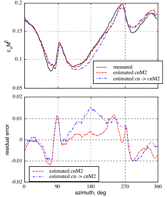
Fig. 24. Measured versus estimated airloads c_n M^2 (LH3-nn-model without azimuth angle input) and residual error as function of azimuth angle for database subset #7 (0.90R, \alpha=-10^\circ , C_T/\sigma=0.128 )
