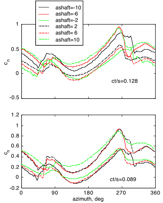
Fig. 1. Measured TRAM helicopter mode airloads for \mu = 0.15 at radial station r = 0.90R .
