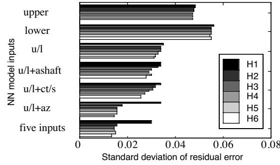
Fig. 15. Goodness of fit for neural network models in estimating airloads c_n at radial station 0.90R using various inputs (pressures at 3.5% chord)
