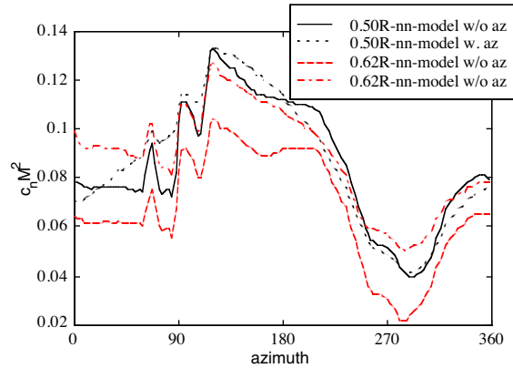
Fig. 36. Airloads estimation at intermediate station 0.56R ( \alpha=-2^\circ , c_T/\sigma=0.089 )
