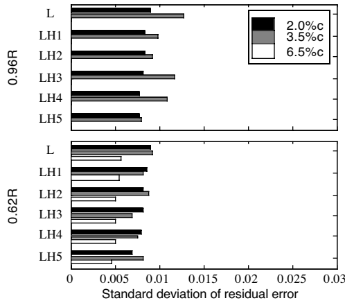
Fig. 27. Goodness of fit for various LHi neural network models in estimating airloads c_n M^2 at two radial stations (inputs: upper/lower surface pressures at 2%, 3.5%, or 6.5% chordwise station, \alpha , and C_T/\sigma )
