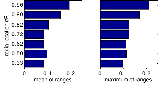
Fig. 22. Mean of ranges and maximum range of airloads c_n for considered test points for seven radial locations
