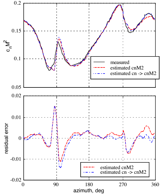
Fig. 25. Measured versus estimated airloads c_n M^2 (LH3-nn-model with azimuth angle input) and residual error as function of azimuth angle for database-subset #7 (0.90R, \alpha=-10^\circ , C_T/\sigma=0.128 )
