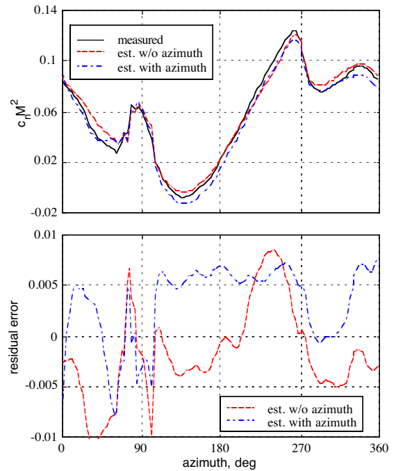
Fig. 28. Measured versus estimated airloads (LH3-nn-model; without and with azimuth angle as input) and residual error as function of azimuth angle for database subset #1 (0.90R, \alpha=-10^\circ , c_T/\sigma=0.089 ); subsets #1 and #7 removed from training database
