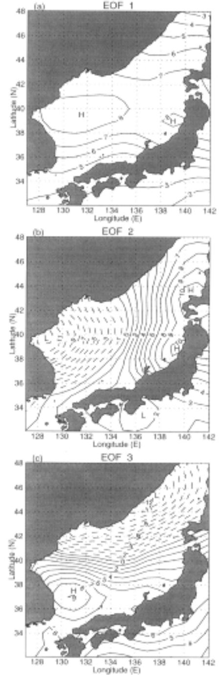
Fig. 8. The first three EOF modes of SST (unit in 0.01^{\circ}\text{C} ): (a) the first EOF, (b) the second EOF, and (c) the third EOF. The solid (dashed) lines indicate positive (negative) values.
