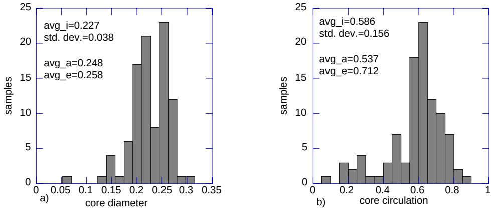
Figure 20. Distribution of instantaneous core quantities for a horizontal cut through a CCW vortex at low thrust, moderate (positive) shaft angle.
