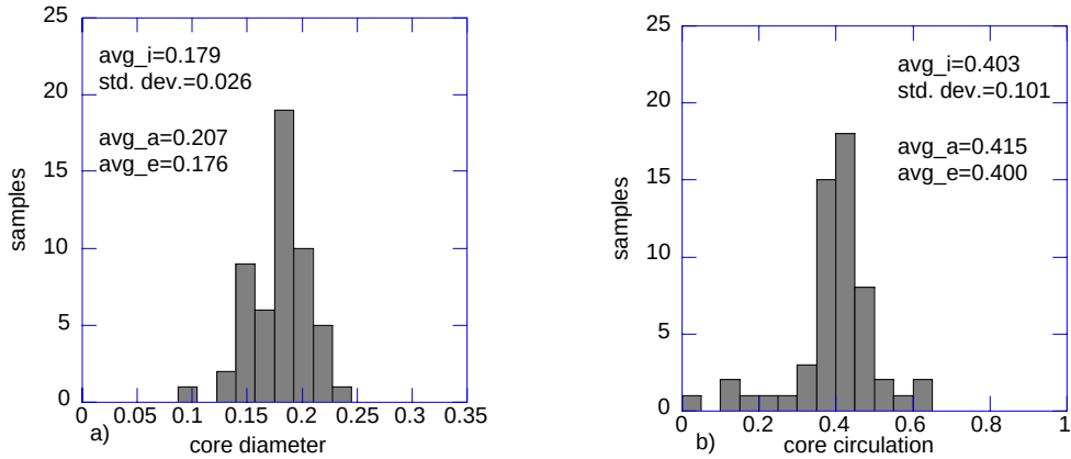
Figure 21. Distribution of instantaneous core quantities for a horizontal cut through a CCW vortex at high thrust, moderate (positive) shaft angle.
