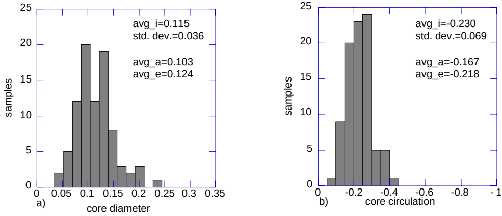
Figure 19. Distribution of instantaneous core quantities for a horizontal cut through a CW vortex at low thrust, moderate (positive) shaft angle.
