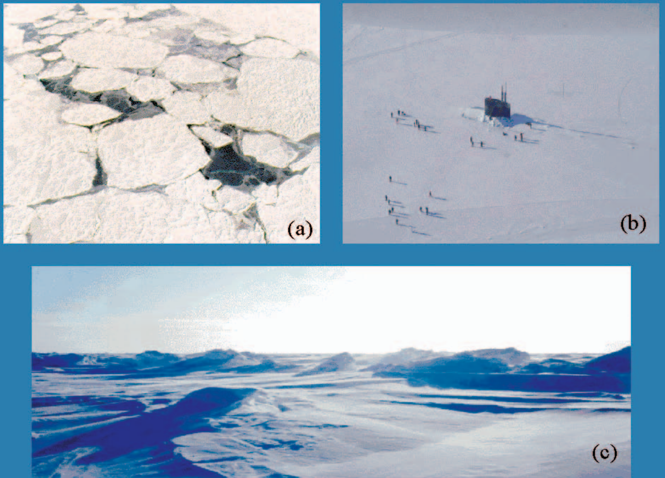
Figure 1. Different forms of sea ice: a) ice floes, b) a level field of solid sea ice penetrated by the sail of the submarine USS Hawkbill, SCICEX '99 and c) ridged ice. Figures are courtesy of a) the Canadian Ice Services, b) the Arctic Submarine Laboratory and c) Ms. Sigrid Salo of NOAA.
