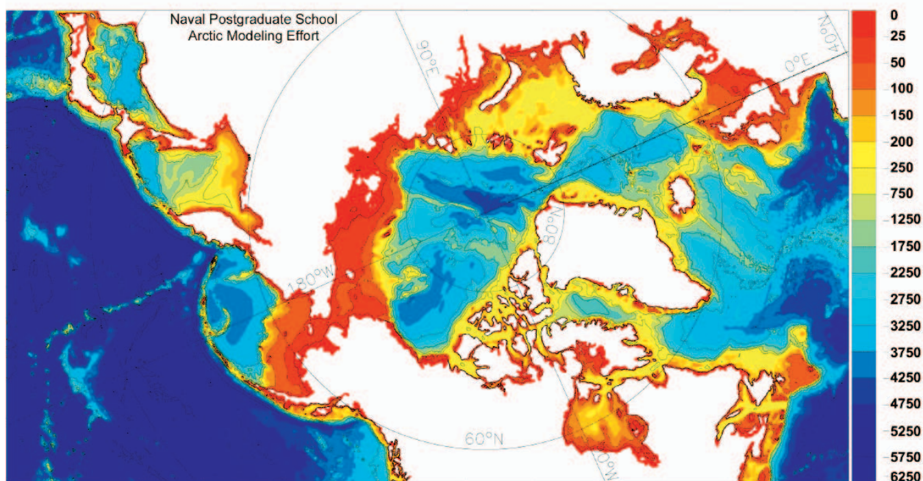
Figure 6. \frac{1}{12} degree, high resolution, coupled model domain and bathymetry. Contours of 25, 50, 100, 500, 1000, 2000, 3000, 4000, 5000 and 6000 m isobaths are shown. More information about the model is available at http://www.oc.nps.navy.mil/~pips3 .
