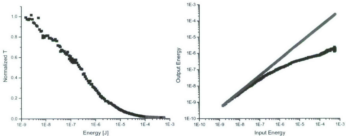
Figure B2. Experimental data for thick sample limiting experiment using F=3.5” D≈10mm F# ≈ 8.89.
