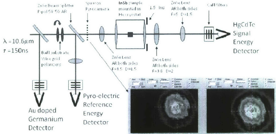
Figure B1. Experimental schematic for thick sample limiting experiment using F=3.5” D≈10mm F# ≈ 8.89.
