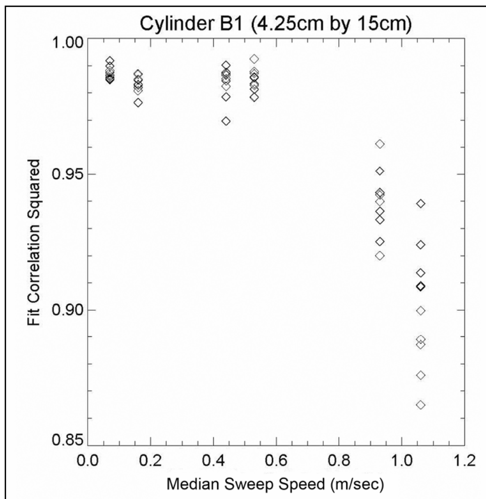
Figure 20. Quality of dipole-fit analysis as a function of sweep speed.
