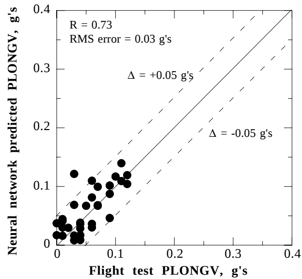
Fig. 36b. Validation plot, five inputs including hub accelerations, advance ratio and gross weight, associated with Fig. 34.
