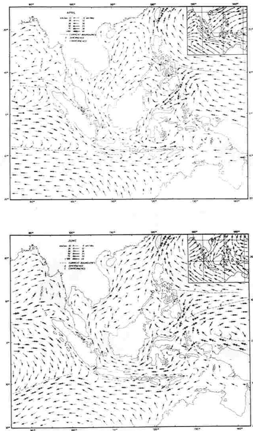
Figure 2. A drastic change of the surface circulation from (a) April to (b) June [after Wyrski, 1961].
