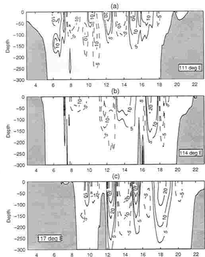
Figure 14. Distribution of velocity u component at several meridional cross sections: (a) 111°E, (b) 114°E, and (c) 117°E.
