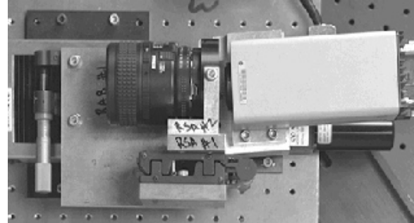
Fig. 6. Photograph of the camera assembly.
