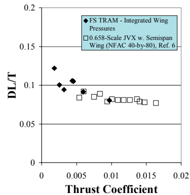
Fig. 10 – Qualitative Data Comparison Between Tiltrotor Hover Download Tests/Configurations
