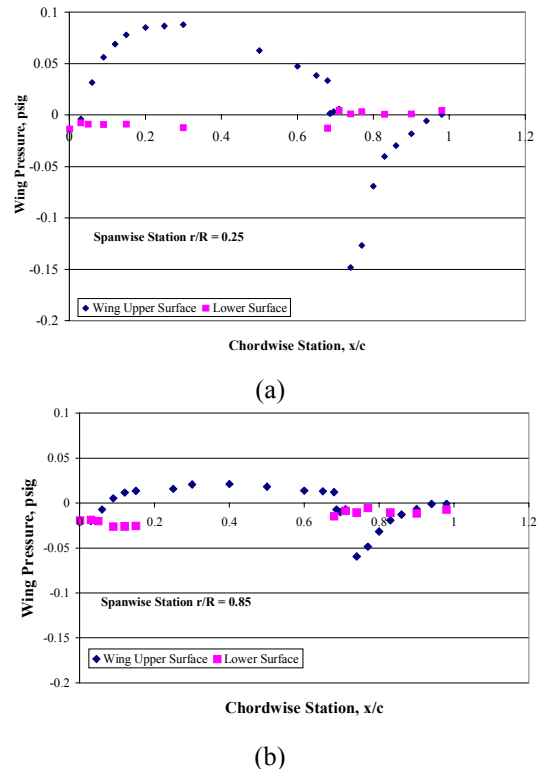
Fig. 8a-b– Sample of Wing Chordwise Pressure Distributions ( C_T = 0.0046 )
