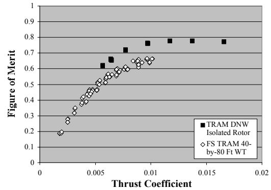
Fig. 7 – Influence of Wing/Airframe on Rotor Hover Performance
