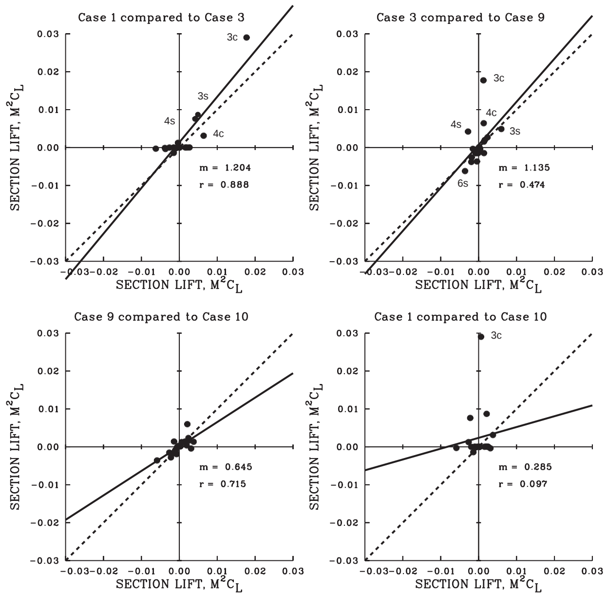
Figure 2. – Harmonic correlation showing stepwise comparisons between cases for Westland/DERA analysis; 3–12 harmonics.
