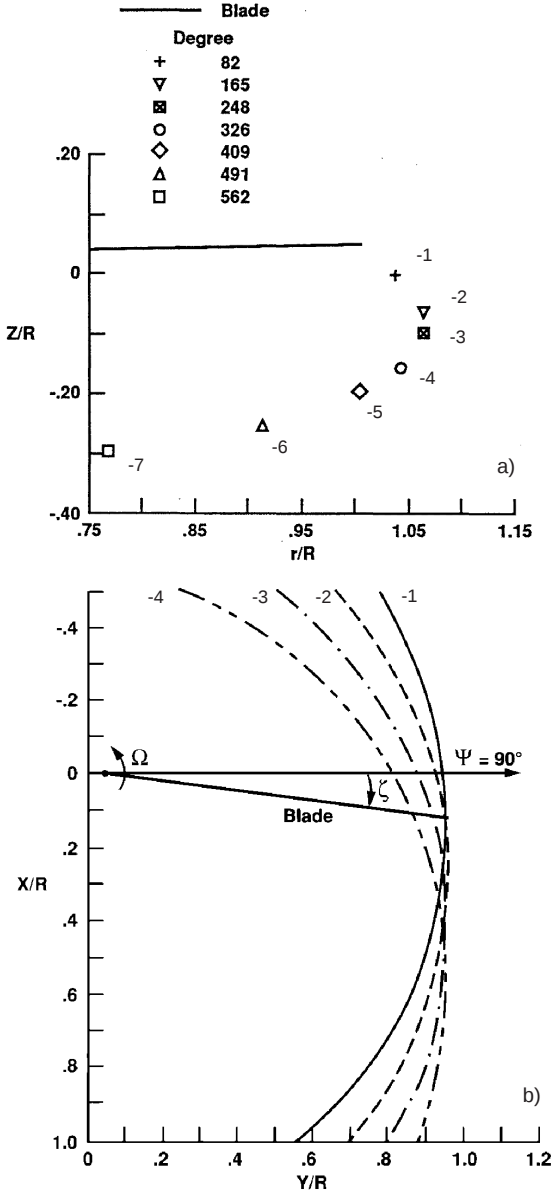
Figure 4. – Calculated tip vortex positions using a prescribed wake for the research Puma at \mu = 0.098 (Ref. 9). a) View in cutting plane at \psi = 75^\circ . b) View in disc plane.
