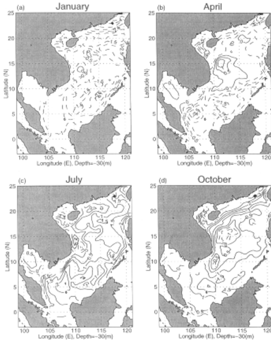
Fig. 8. Monthly temperature anomaly at 30-m depth for the control run: (a) January, (b) April, (c) July, and (d) October. Here, the solid (dashed) curves denote positive (negative) values.
