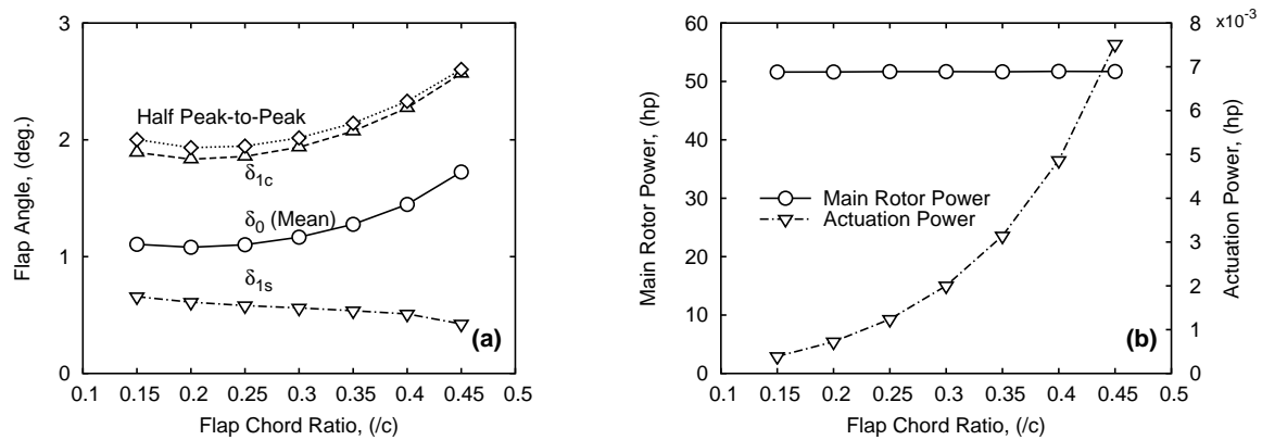
Figure 7: Effect of trailing-edge flap chord ratio on flap angles, main rotor power, and and actuation requirements at forward speed of 60 knots ( \mu = 0.16 )
