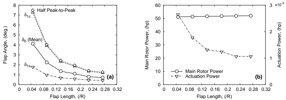
Figure 6: Effect of trailing-edge flap length on flap angles, main rotor power, and and actuation requirements at forward speed of 60 knots ( \mu = 0.16 )
