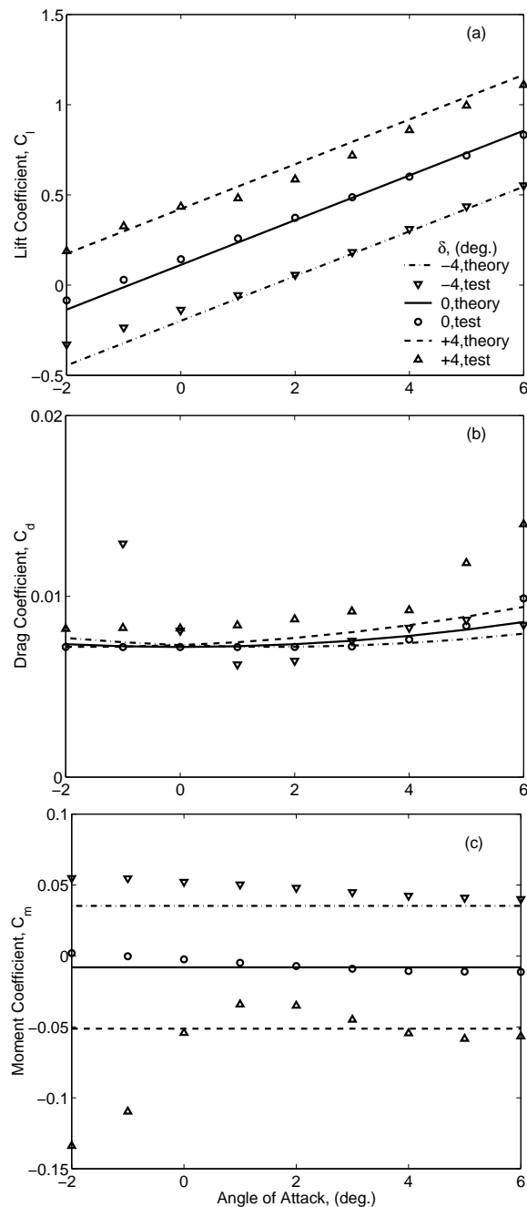
Figure 1: Measured and predicted aerodynamic coefficients of 2D HH-06 airfoil with 0.35 plain trailing-edge flap (10% chord overhang, Mach = 0.45); (a) lift (b) drag and (c) pitching moment
