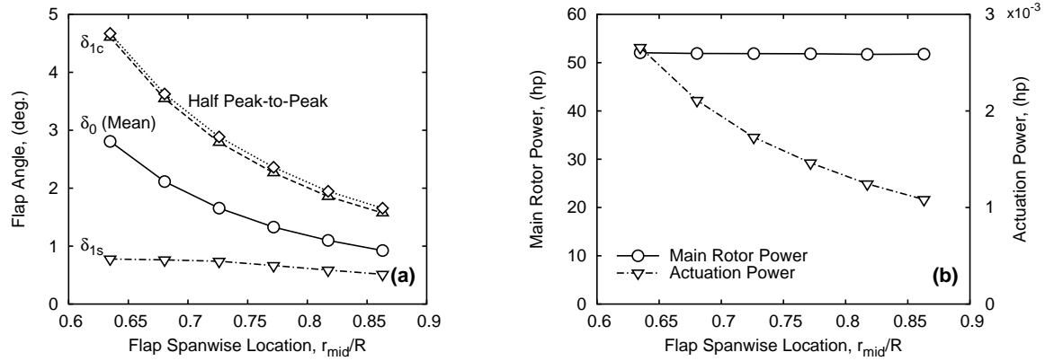
Figure 5: Effect of trailing-edge flap location on flap angles, main rotor power, and and actuation requirements at forward speed of 60 knots ( \mu = 0.16 )
