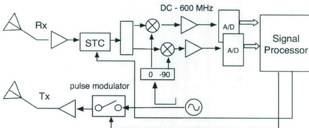
Figure 8. Simplified Block Diagram for a pulsed RF carrier type radar. Critical component technologies in this type of radar are the STC circuit, the A/Ds, and the pulse modulator.
