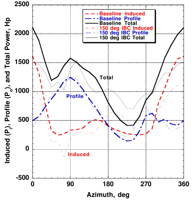
Figure 5: Profile and induced power on a helicopter with 3 deg IBC, 180 kts, C_T/\sigma=0.092 , Army hot day
