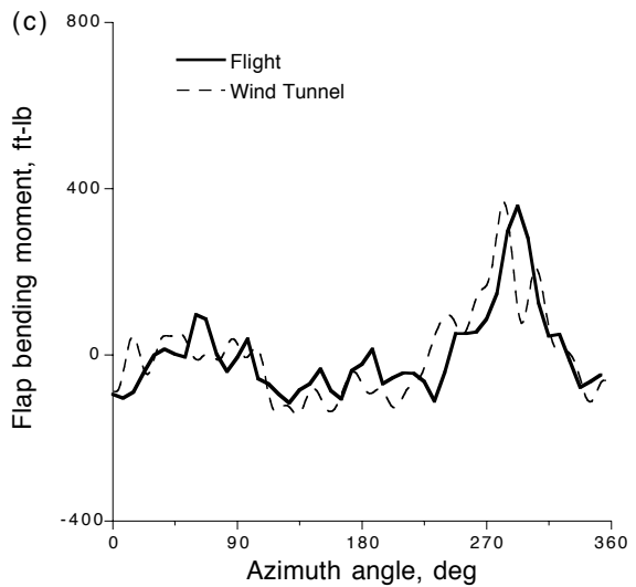
Figure 25. Comparison between flight and wind tunnel tests of oscillatory flap bending moments at (a) r/R=0.5 , (b) r/R=0.7 , (c) r/R=0.9 , ( \mu=0.178 , C_T/\sigma=0.08 ).
