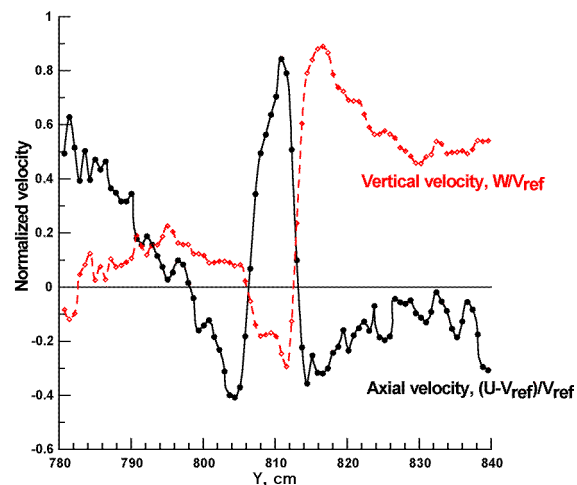
Figure 27. Normalized axial and vertical velocity profiles through the primary tip vortex core, looking downstream ( \mu=0.150 , M_{TIP}=0.650 , C_T/\sigma=0.08 , \alpha_s=0 deg, 15 deg wake age).
