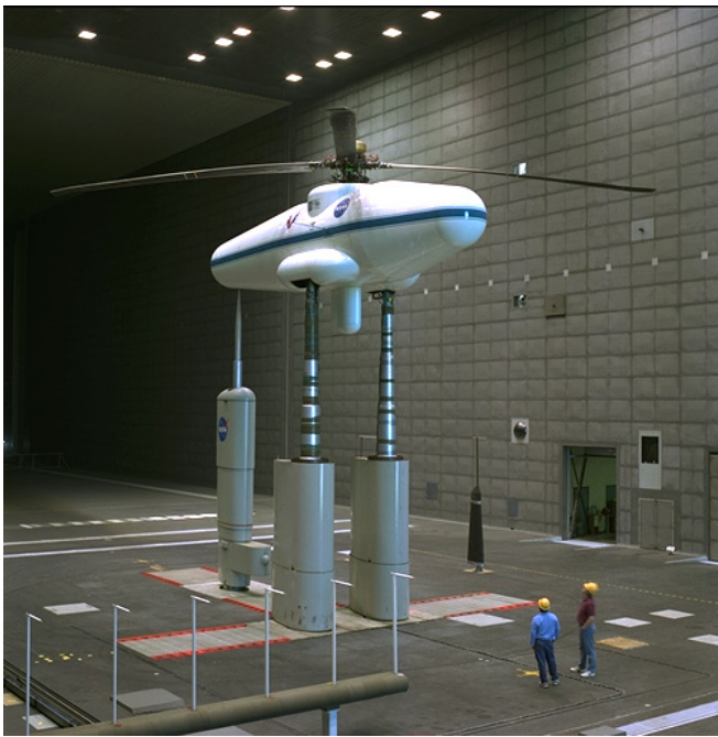
Figure 1. UH-60 Rotor System installed on the Large Rotor Test Apparatus in the Ames 80-by 120-Foot Wind Tunnel.
