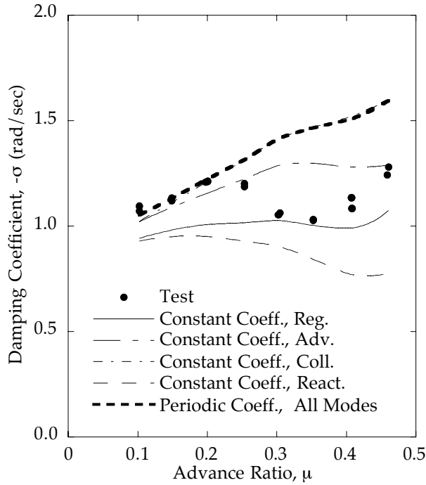
Fig. 18 Comparison with swept-tip rotor of measured forward flight regressing lag mode damping, and 2 CAMRAD II solution methods; 0° shaft angle, 6° collective pitch angle, 0° precone hub.
