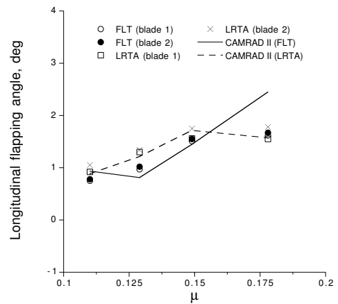
(b) Longitudinal flapping angle
