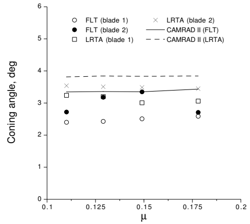
(a) Coning angle
