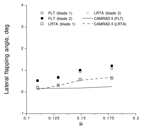
(c) lateral flapping angle
