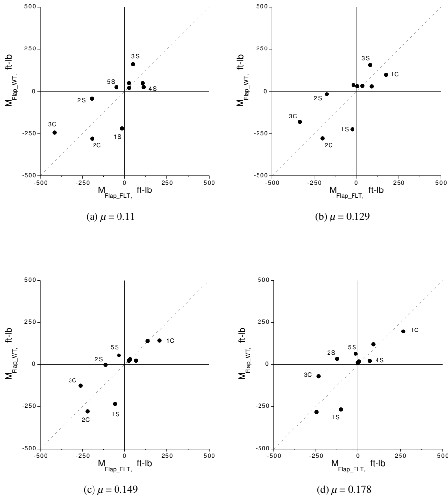
Fig. 14 Harmonic comparison of flap bending moment between flight and wind tunnel test at r/R = 0.7
