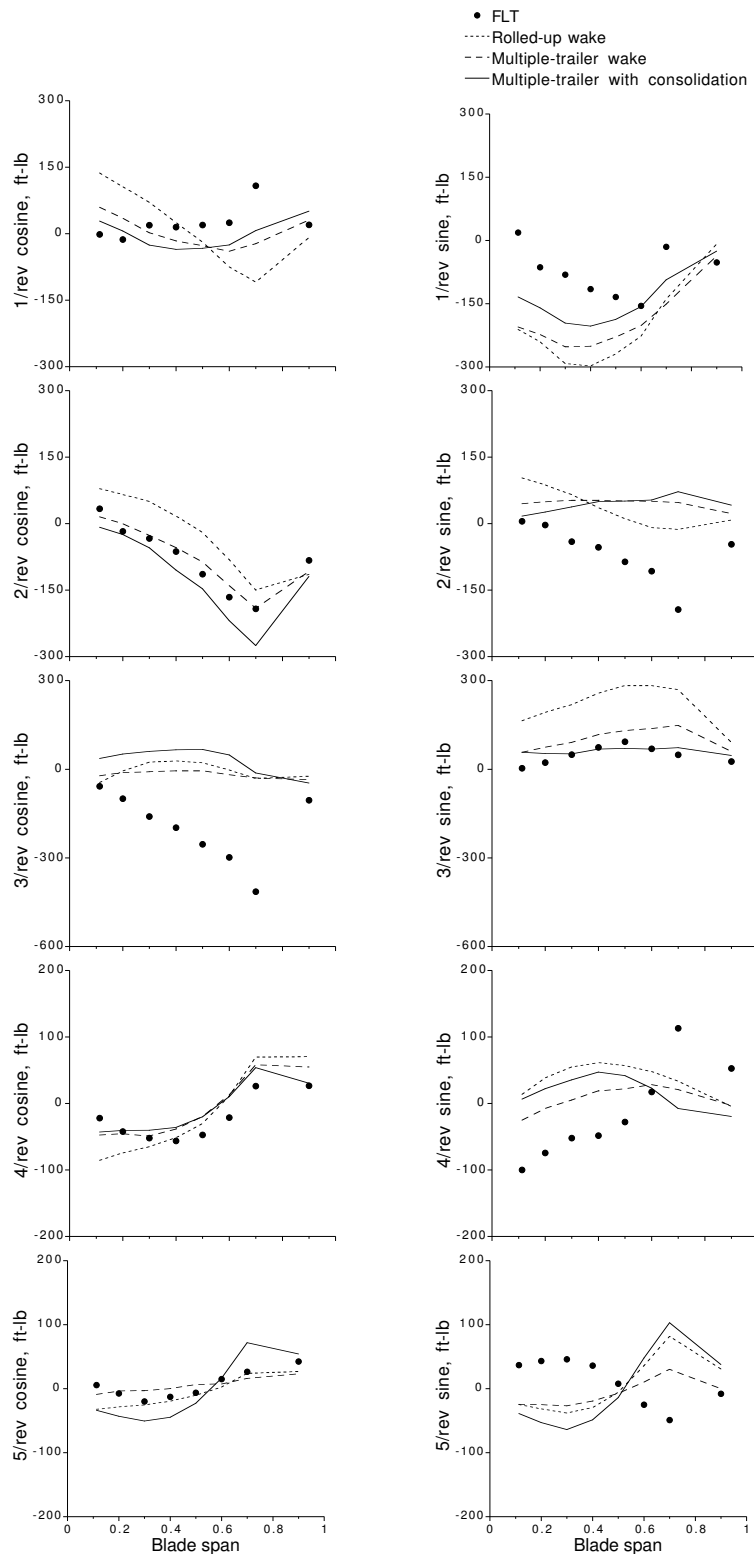
Fig. 19 Comparison of cosine and sine harmonics of flap bending moment with flight test data for \mu = 0.11
