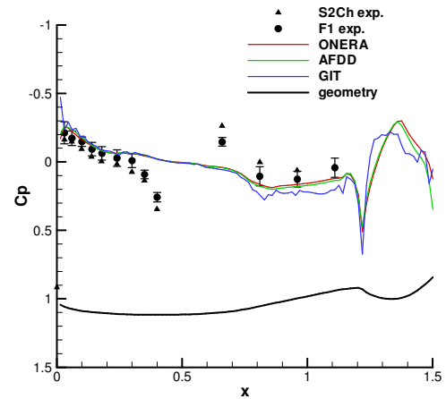
b) lower fuselage centerline
