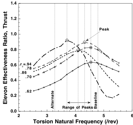
Figure 5. Effect of torsion natural frequency on elevon 4/rev thrust force effectiveness for various elevon radial positions, normalized by baseline ( \omega_{\phi 1} = 4.79/\text{rev} ) steady-state 4/rev thrust at \mu = 0.125 .
