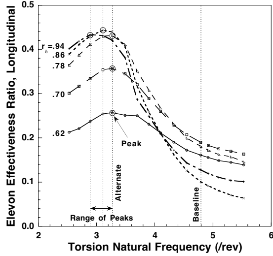
Figure 4. Effect of torsion natural frequency on elevon 4/rev longitudinal force effectiveness for various elevon radial positions, normalized by baseline ( \omega_{\phi 1} = 4.79/\text{rev} ) steady-state 4/rev longitudinal force at \mu = 0.125 .
