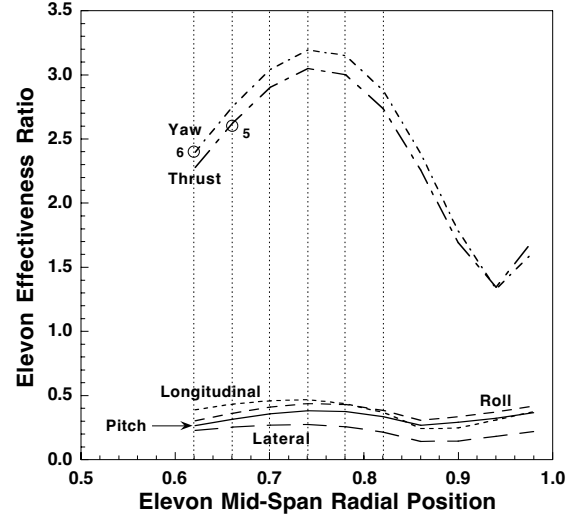
Figure 6. Effect of elevon radial position on elevon effectiveness for reducing 4/rev hub loads for the baseline ( \omega_{\phi 1} = 4.79/\text{rev} ); each hub load is normalized by its corresponding ( \omega_{\phi 1} = 4.79/\text{rev} ) steady-state vibratory load at \mu = 0.25 .
