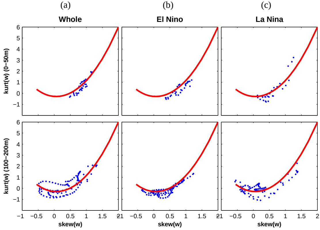
4 Fig. 3. Relationship between kurt(w) and skew(w) for the observational w -PDFs (dots) from 5 TAO-ADCP at the six stations and the Weibull distribution (solid curve) during (a) the whole 6 period, (b) major El Nino events, and (c) major La Nina events with the upper panels for the 7 upper layer (0-50 m), and the lower panels for the sub-layer (100-200 m).
