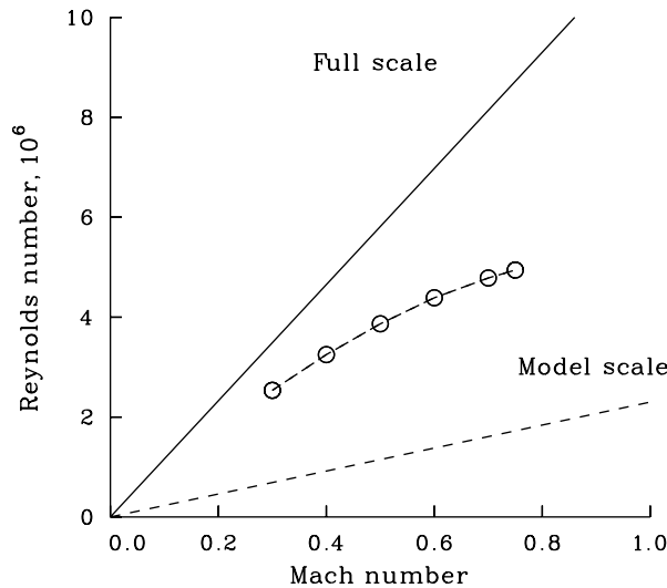
Figure 9. Test conditions for experiment 2; TSW in the UTRC Large Subsonic Wind Tunnel (ref. 3).
