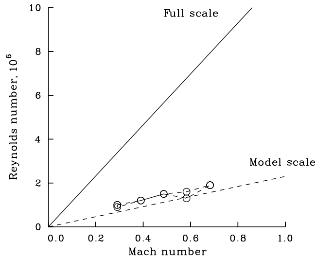
Figure 12. Test conditions for experiment 4; NRC (Canada) 12- by 12-Inch Icing Wind Tunnel (ref. 5).
