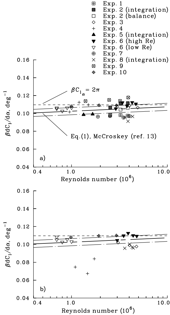
Figure 23. Lift-curve slope at zero lift as a function of Reynolds number; all experimental datasets, M < 0.55 . a) SC1095 airfoil; b) SC1094 R8 airfoil. \beta C_{l_\alpha} reference lines for NACA 0012 (ref. 13).
