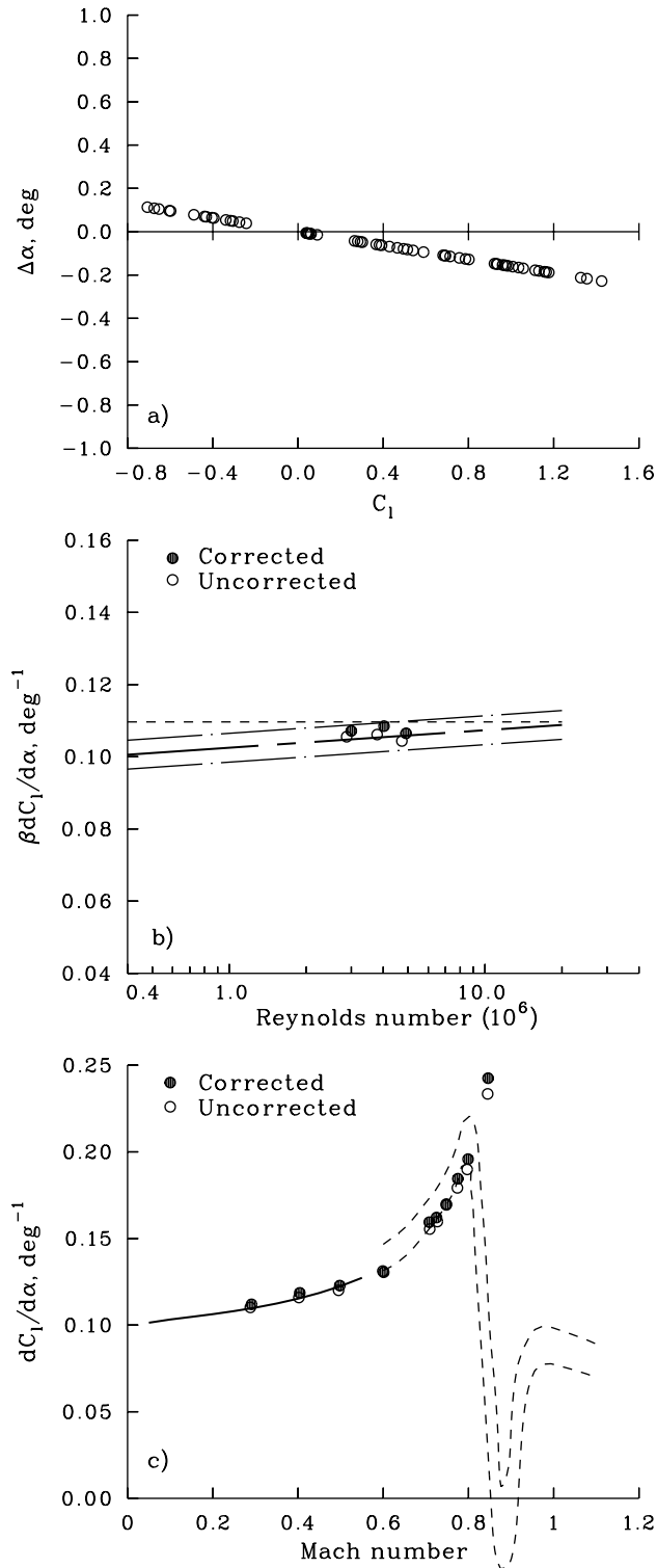
Figure 11. Comparison of corrected and uncorrected data for experiment 3. \beta C_{l\alpha} and C_{l\alpha} reference lines for NACA 0012 (ref. 13).
