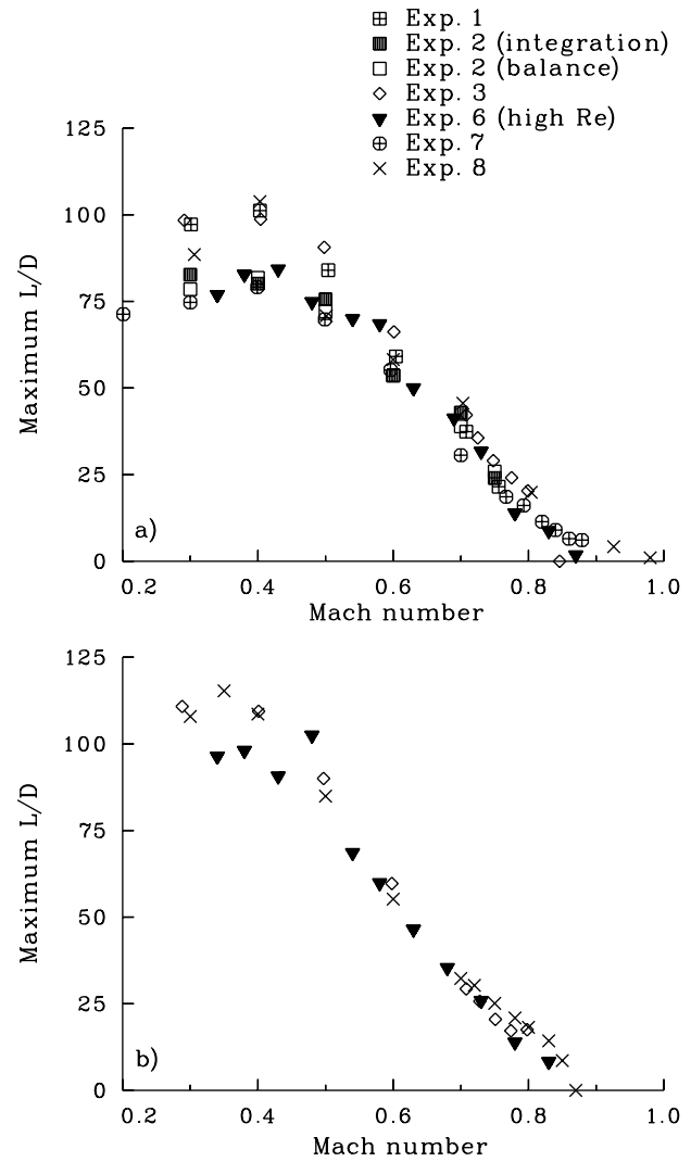
Figure 37. Maximum L/D as a function of Mach number; a) SC1095 airfoil; b) SC1094 R8 airfoil.
