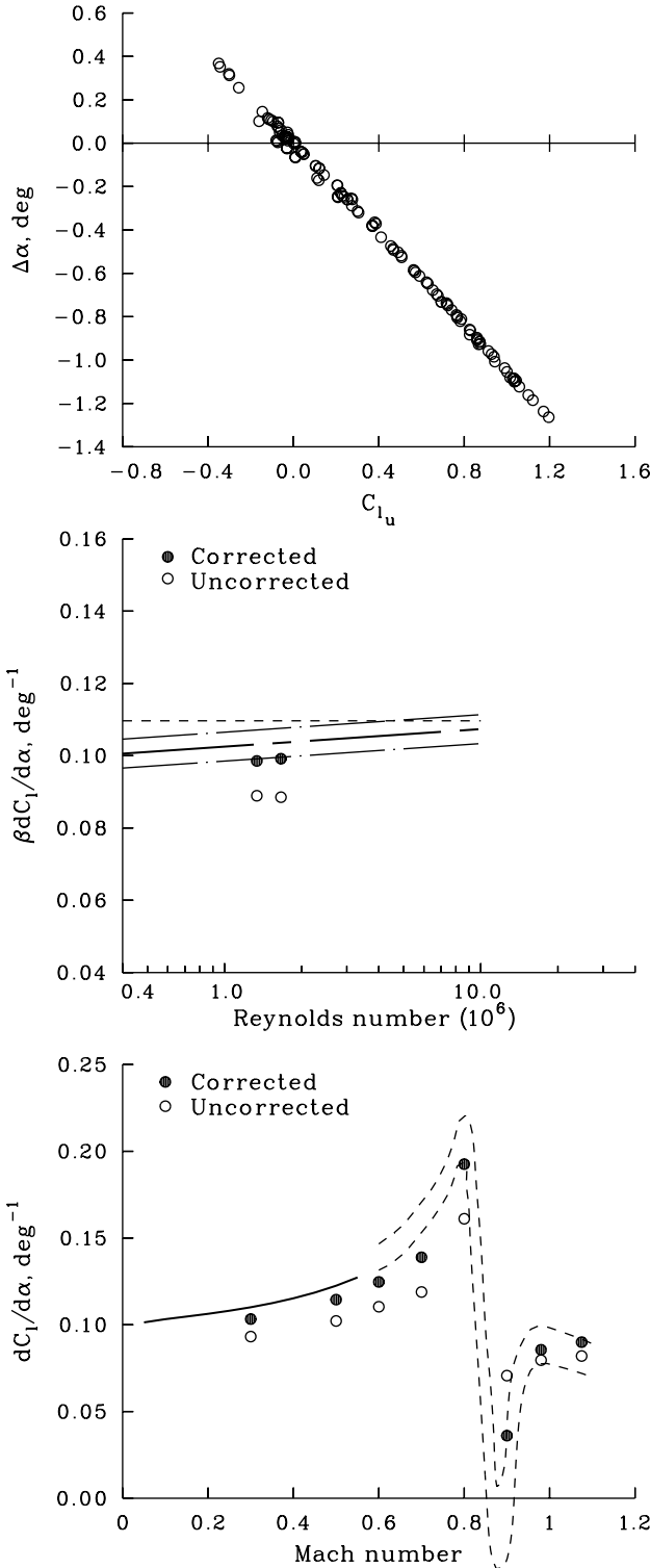
Figure 14. Comparison of corrected and uncorrected data for experiment 5. \beta C_{l\alpha} and C_{l\alpha} reference lines for NACA 0012 (ref. 13).
