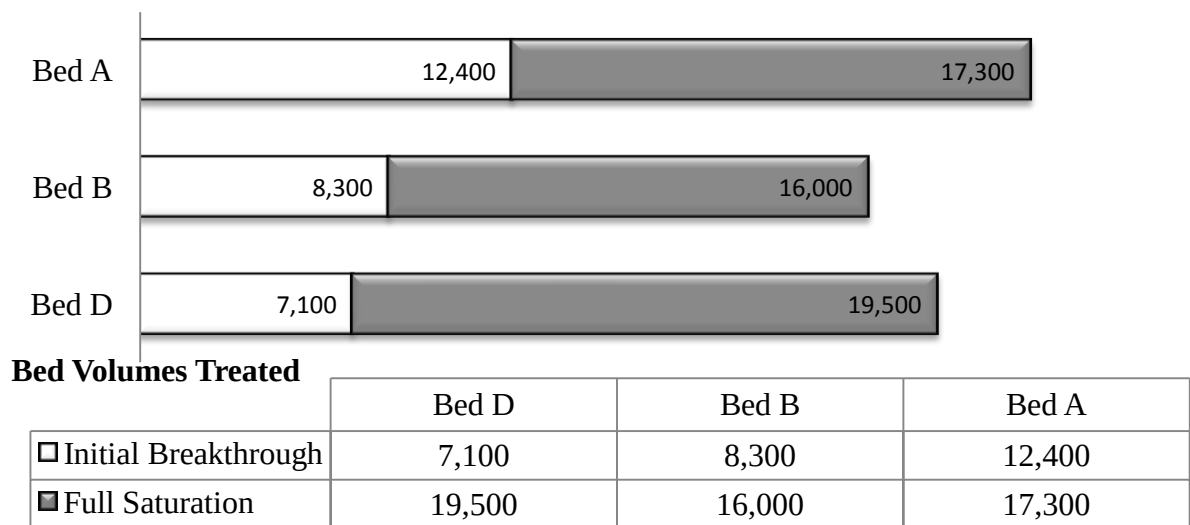
Figure 4-5. Fontana Pilot-Scale Column Performance (37 GPM)
