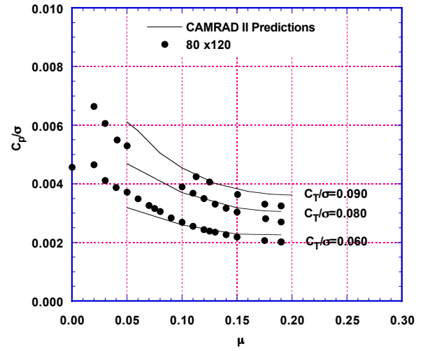
Fig. 30. Measured and calculated rotor power vs. advance ratio for various thrust conditions, \alpha_s = 0^\circ , M_{TIP} = 0.650 .
