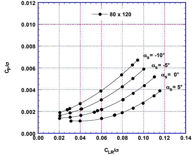
Fig. 15. Measured 80 x 120 rotor power vs. rotor lift for various rotor shaft angles at an advance ratio of 0.150, M_{TIP} = 0.650 .
