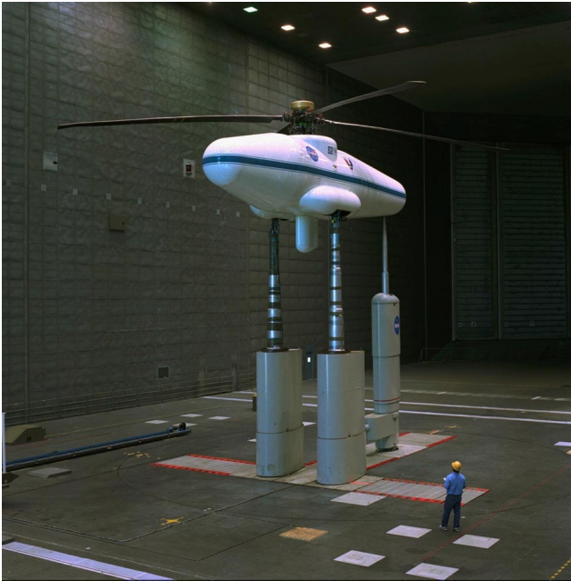
Fig. 1. UH-60 Rotor System installed on Large Rotor Test Apparatus in the Ames 80- by 120-Foot Wind Tunnel.
