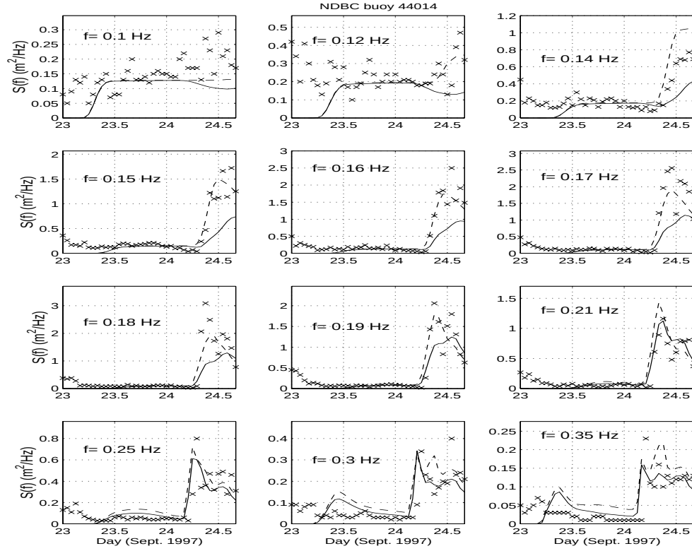
Figure 6. Comparison of SWAN frequency spectra time series to data from NDBC buoy 44014. “x”: data; solid line: model with n=1.5 ; dashed line: model with n=1.5 , without breaking of swell, as defined in (3).
