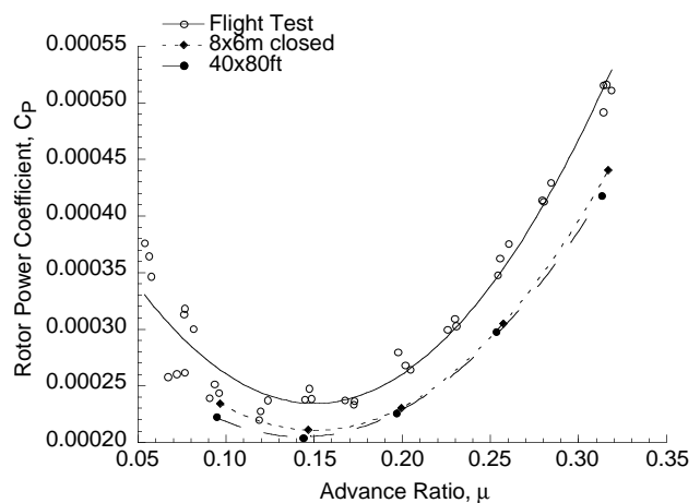
Figure 38. Comparison of model- and full-scale rotor power as a function of advance ratio without propulsive force trim or wall induced corrections with flight test measurements.
