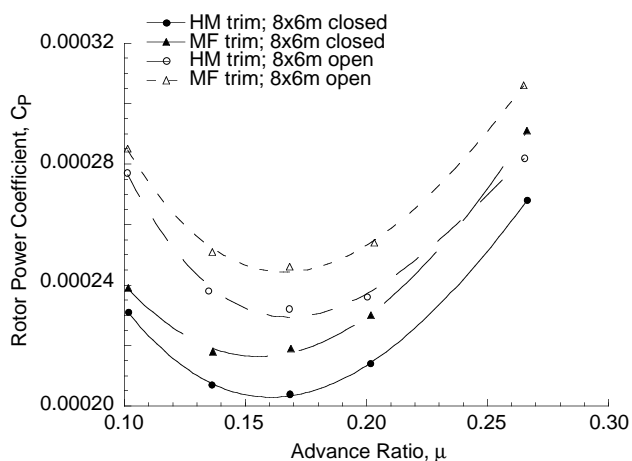
Figure 15. Comparison of rotor power as a function of advance ratio for minimized flapping (MF) and hub moment (HM) trim, c_T = 0.005 .
