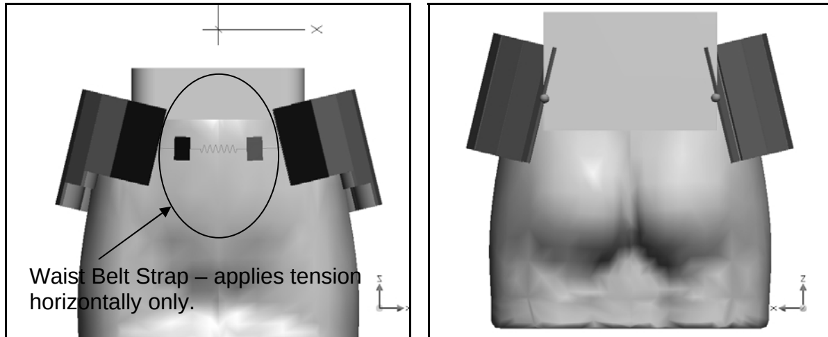
Figure 19: Spherical constraints – effect on ability of belt to conform. Front view (left) and back view (right). Hip pads are allowed to penetrate lumbar pad to ensure good fit.
