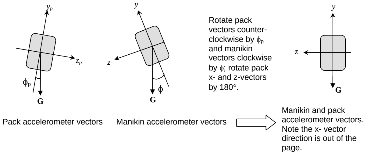
Figure 10: Rotation of manikin and pack vectors into global coordinate system. Rotation is based on aligning the gravity vector, G .
