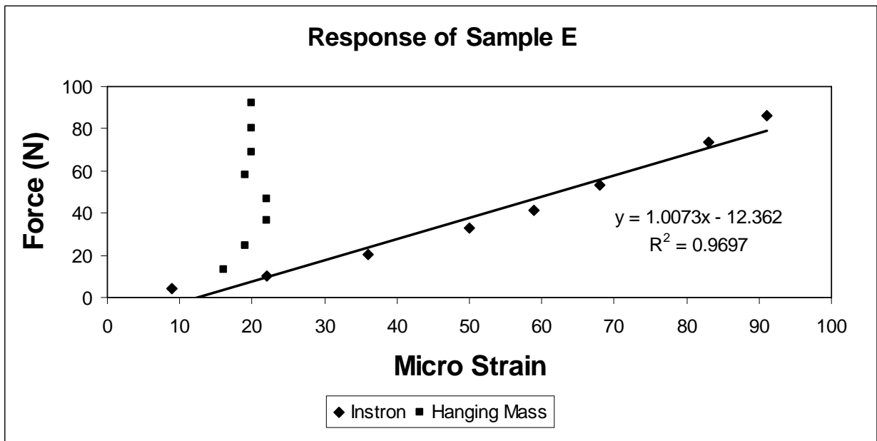
Figure G4: Sample E, Al 6061-T6, (1", 350Ω, half bridge, t=1.727)
