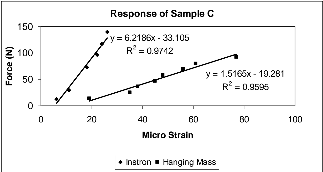
Figure G3: Sample C, Al 6061-T6, (1000 Ω, half bridge, t=1.676 mm)
