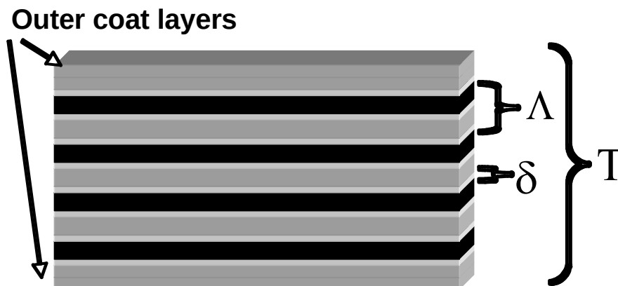
Scheme 1. Scheme showing the structural features of an energetic multilayer. The distance T_t is the total thickness of the multilayer, \Lambda is the period or the repeating structural unit of the multilayer, and \delta is the prereaction zone
