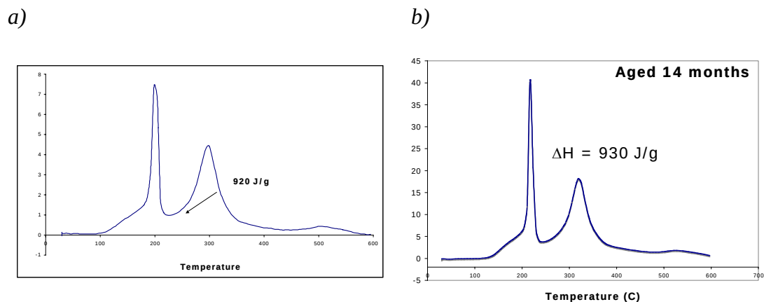
Figure 5. DSC traces for uncoated Al/Ni(V) films right after fabrication a) and after 14 months of storage under ambient conditions.
