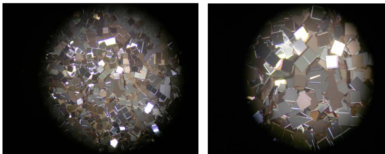
Figure 8. Photos of uniform powderized Al/Ni(V) nanolaminate. The particles are 300 μm x 300 μm.
