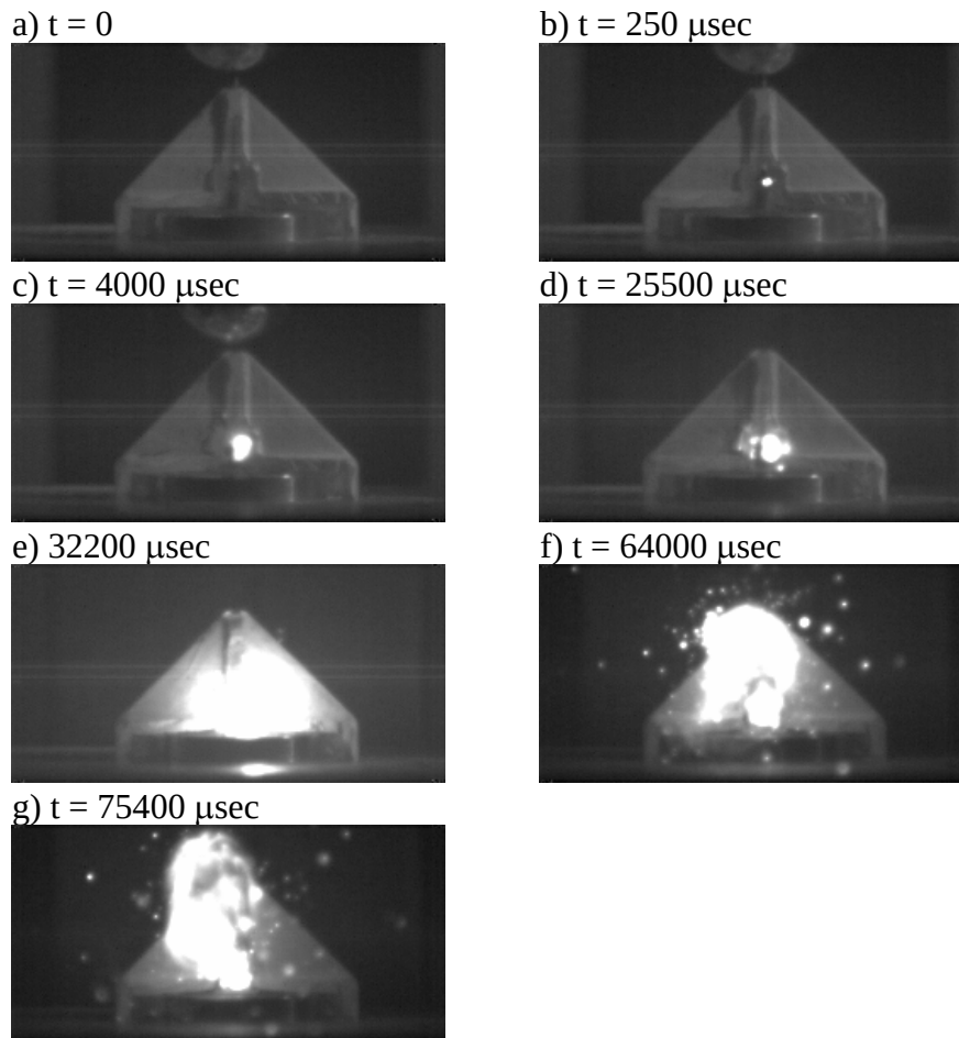
Figure 15. Series of photos from high-speed images of stab initiation of energetic multilayers and subsequently igniting thermite material.
