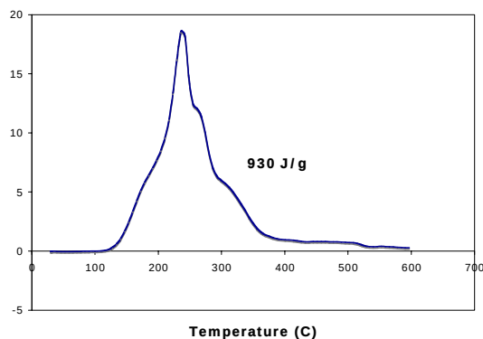
Figure 6. DSC of uncoated Al/Monel energetic multilayer 14 months after fabrication.
