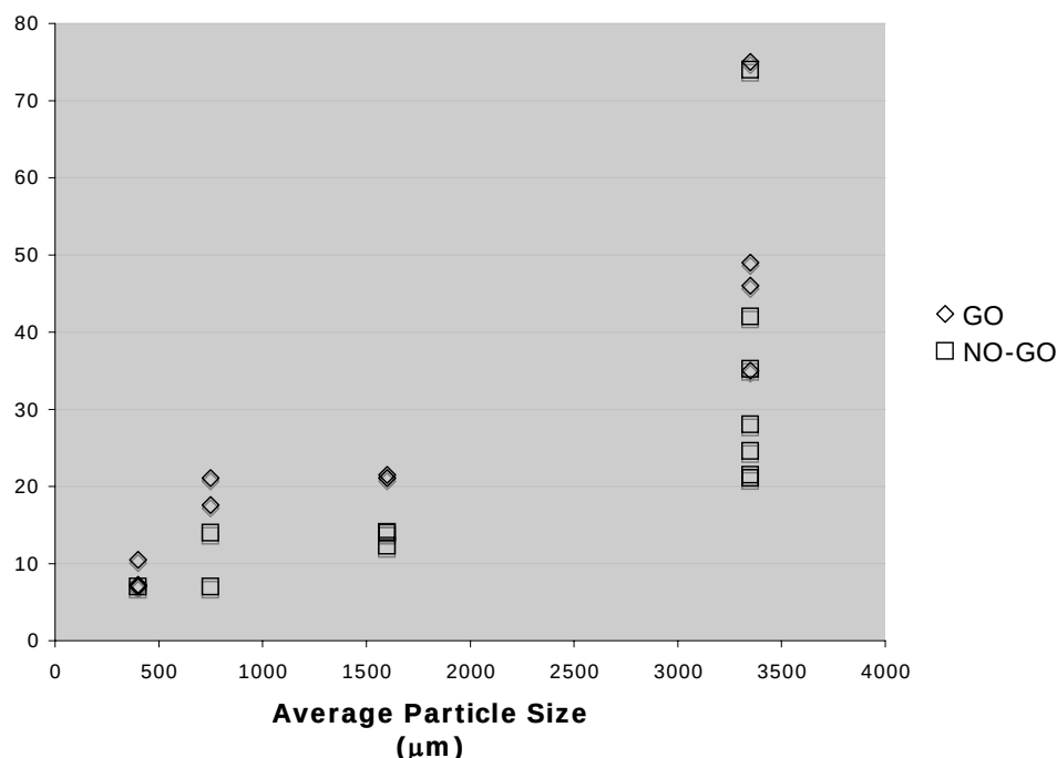
Figure 11. Plot of impact energy versus average particle size for an uncoated Al/Monel 400 multilayer material with a 20 nm bi-layer period, an overall thickness of 55 \mu\text{m} , and tested in configuration B (see Scheme 2 for clarification).
