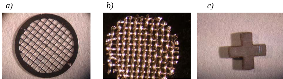
Figure 14. Photos of mesh media a) and b) and cross (c) used to enhance pinching interactions with the energetic multilayer in stab detonator configurations. The diameter of each structure is nominally 3 mm.
