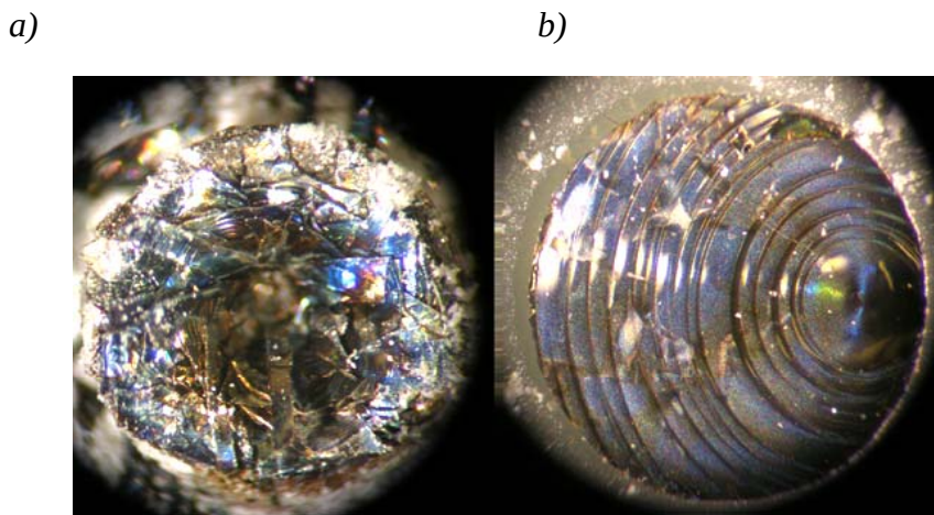
Figure 9. Photos of successful (go) reacted multilayer energetic foils materials. These materials were initiated in a M55 mock detonator configuration with stab input.
