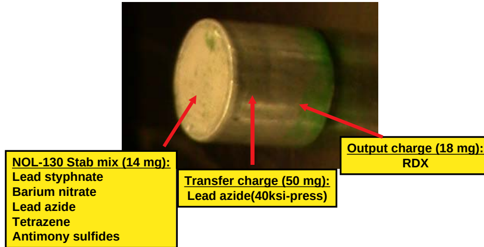
Figure 1. Photo of M55 stab detonator Al cup with initiation train and components.
