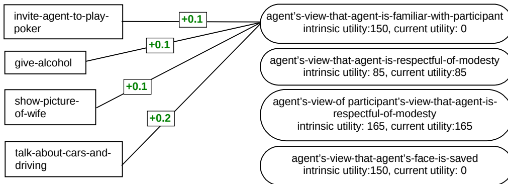
Figure 3 Sample of Socio-Cultural Network for German Culture
