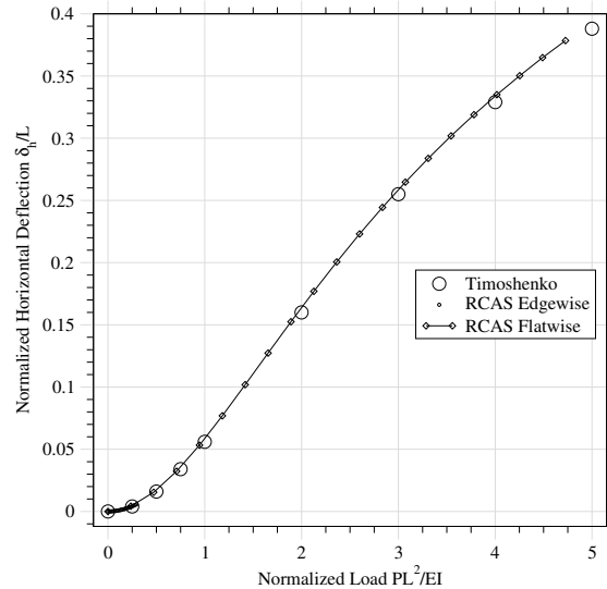
Figure 12: Tip Loaded Elastica: Horizontal Displacement, \delta_h vs. RCAS for L = 20\text{in} , N = 8 , P = 0.5 \dots 10\text{lb} and EI = 8.463 \times 10^2 or 1.354 \times 10^4\text{lb/in}^2 .
