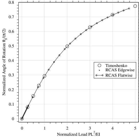
Figure 10: Tip Loaded Elastica: Rotation Angle, \theta_b vs. RCAS for L = 20\text{in} , N = 8 , P = 0.5 \dots 10\text{lb} and EI = 8.463 \times 10^2 or 1.354 \times 10^4\text{lb/in}^2 .
