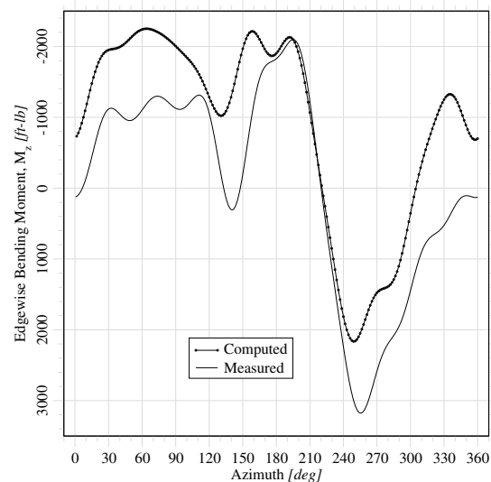
Figure 26: UH-60 blade edgewise bending moment, 11.3% R.
