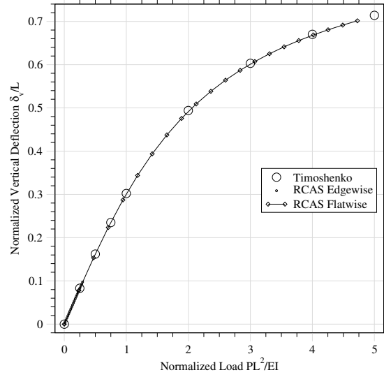
Figure 11: Tip Loaded Elastica: Vertical Displacement, \delta_v vs. RCAS for L = 20\text{in} , N = 8 , P = 0.5 \dots 10\text{lb} and EI = 8.463 \times 10^2 or 1.354 \times 10^4\text{lb/in}^2 .
