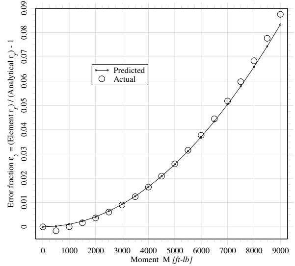
Figure 3: Relative intrinsic element error: predicted vs. actual RCAS error at the end of the first element with L = 20\text{ft} , s = 1\text{ft} , EI = 9000\text{lb-ft}^2 , and N = 20 .
