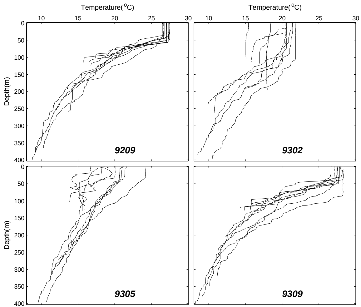
1 2 Figure 17. Temperature profiles in the Tsushima Warm Current branching region (inside 3 the box indicated in Fig. 16).
