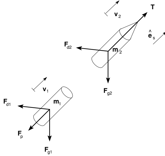
Figure 1. Free-body diagram of the two-stage system after separation. Subscript 2 denotes the upper stage and subscript 1 denotes the lower stage.
