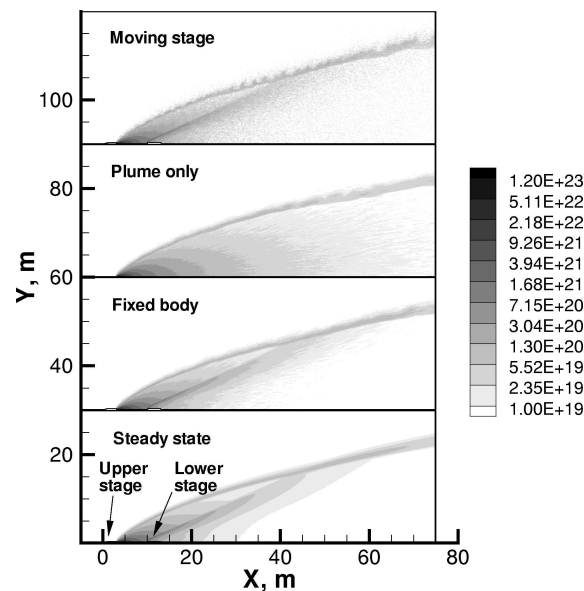
Figure 3. Liquid propellant thruster: plume \text{H}_2\text{O} number density fields ( \text{mol}/\text{m}^3 ) at 0.3 s after thruster ignition.
