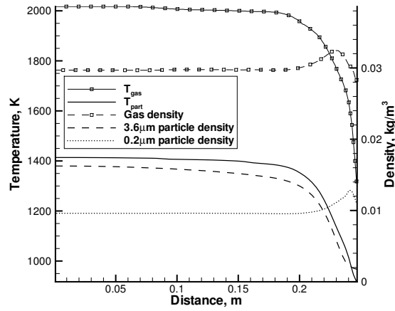
Figure 9. Solid propellant thruster: flow properties across the nozzle exit plane.
