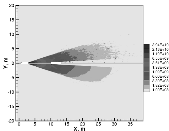
Figure 11. Solid propellant: number density fields (molecule/m 3 ) of large particulates at 0.3 seconds after separation. The top half is the unsteady results and the lower half is the steady state results.
