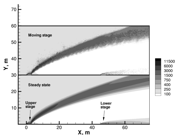
Figure 4. Liquid propellant thruster: translational temperature fields (K) at 1.0 s after thruster ignition.
