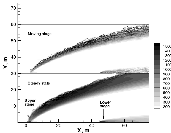
Figure 5. Liquid propellant thruster: vibrational temperature field (K) at 1.0 s after thruster ignition.
