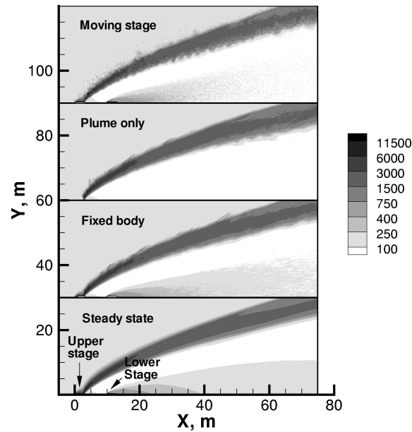
Figure 2. Liquid propellant thruster: translational temperature (K) at 0.3 s after thruster ignition. Here and below, the direction of the free stream velocity is from left to right, going from -x to +x .
