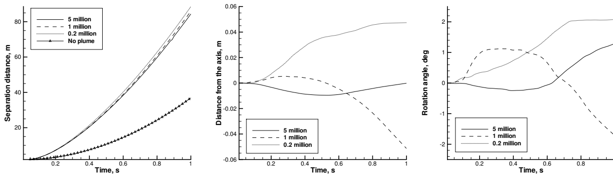
Figure 8. 2D liquid propellant case: the impact of the number of simulated particles on stage separation distance (left), deviation from the plume axis (center), and the rotation angle (right).
