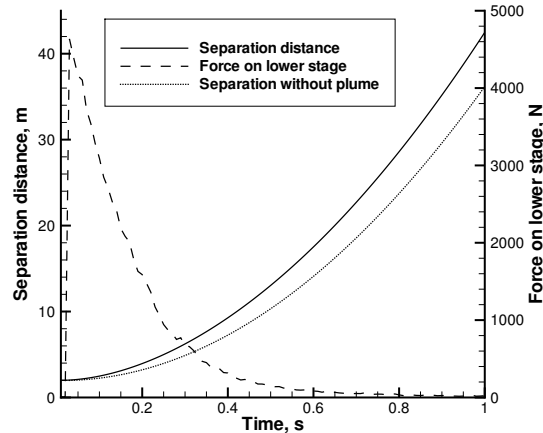
Figure 7. Liquid propellant thruster: temporal profiles of stage separation distance and plume force on lower stage.
