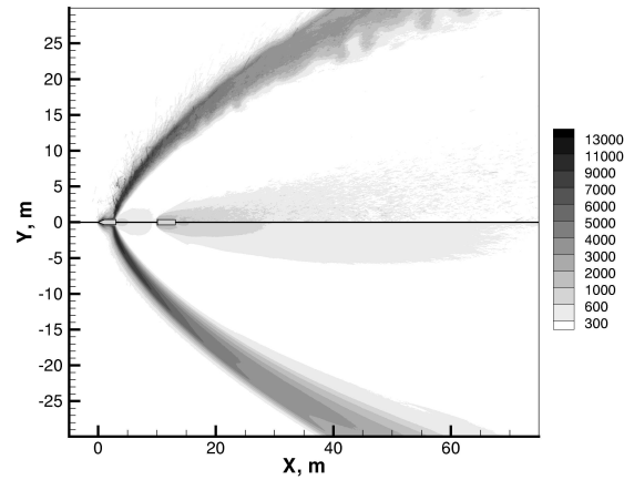
Figure 10. Solid propellant thruster: gas translational temperature (K) at 0.3 s after thruster ignition. The top half are the unsteady results and the bottom half are the steady-state results.
