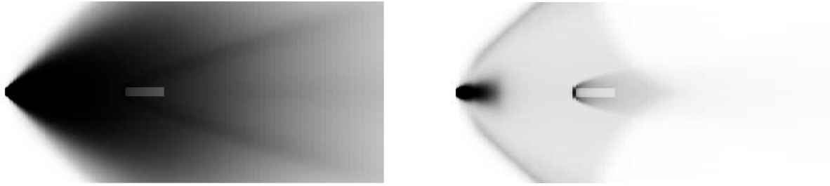
Figure 6. Infrared images of the liquid-propellant staging, as computed with SOCRATES-P for 4.7- \mu\text{m} excited CO (left) and 6.3- \mu\text{m} excited \text{H}_2\text{O} (right). The width of each image is 30 m. The intensity scale has been distorted from linear using an image-processing \gamma=0.01 transfer-function to show the radiance enhancement near the lower stage.
