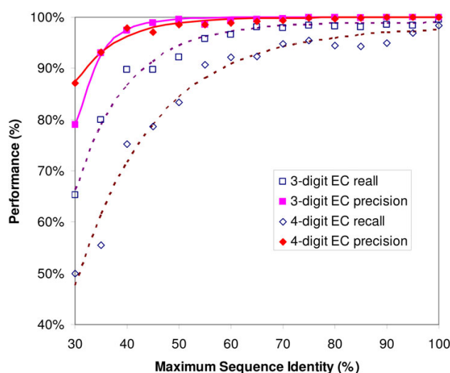
Figure 2 CatFam performance evaluation. The performance of CatFam is measured by precision and recall, which are defined as \text{precision} = \text{TP}/(\text{TP} + \text{FP}) and \text{recall} = \text{TP}/(\text{TP} + \text{FN}) , where TP, FP and FN represent the number of true-positive, false-positive, and false-negative predictions, respectively. A total of 18,949 proteins, not used for profile generation, are used to evaluate two CatFam databases, CatFam-3D and CatFam-4D, which predict 3-digit and 4-digit EC numbers for query proteins, respectively. The results are sorted according to the maximum sequence identity between the query protein and the proteins used for profile generation.
