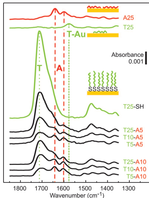
Fig. 2. FTIR spectra obtained from ssDNA adsorbed on gold. The adsorption conditions for the d(T_m-A_5) , d(T_m-A_{10}) , and (dT)_{25} -SH oligos were 3\text{ }\mu\text{M} ssDNA in 1 M \text{CaCl}_2 -TE, pH 7, at 35^\circ\text{C} for 2,400 min. Reference spectra are presented for (dA)_{25} and (dT)_{25} oligo films. The feature at \approx 1,700\text{ cm}^{-1} (green dotted line) corresponds to \text{C}=\text{O} groups in nonchemisorbed dT nucleotides. Features between 1,550 and 1,600\text{ cm}^{-1} (green short dash line) are attributed to chemisorbed dT nucleotides. Features at \approx 1,600 and \approx 1,650\text{ cm}^{-1} (red dashed lines) are associated primarily with dA nucleotides.
