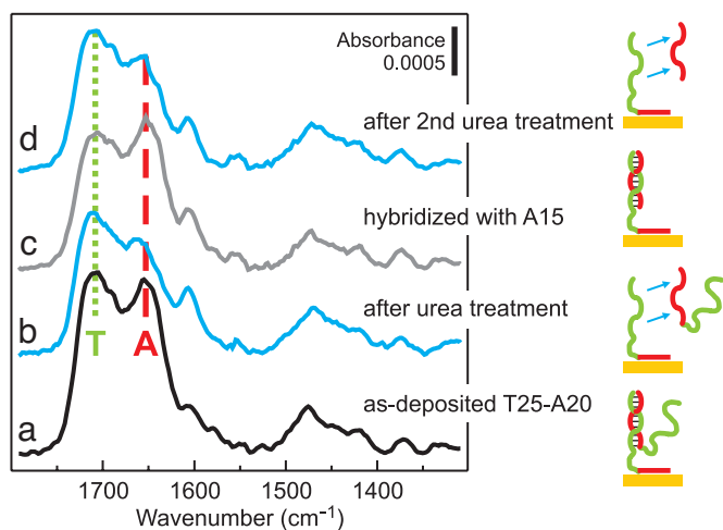
Fig. 7. Hybridization properties of d(T 25 -A 20 ) films. FTIR spectra for d(T 25 -A 20 ) films as deposited (a), after a 30-min soak in 8 M urea denaturing solution (cyan) (b), after a subsequent overnight hybridization with 1 \mu M (dA) 15 in 1 M CaCl 2 -TE buffer (gray) (c), and after a second 30-min soak in 8 M urea (cyan) (d). Spectral features primarily attributed to dT and dA nucleotides are indicated by green dotted and red dashed lines, respectively.
