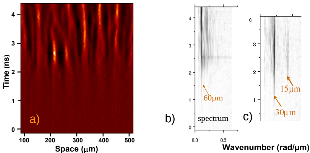
Figure 7. Non-linear interaction of pre-imposed ripple and laser imprint: (a) streak image for \lambda = 60 \mu\text{m} ; (b) time history of the areal mass Fourier spectrum for \lambda = 60 \mu\text{m} ; (c), spectrum for \lambda = 30 \mu\text{m} .
