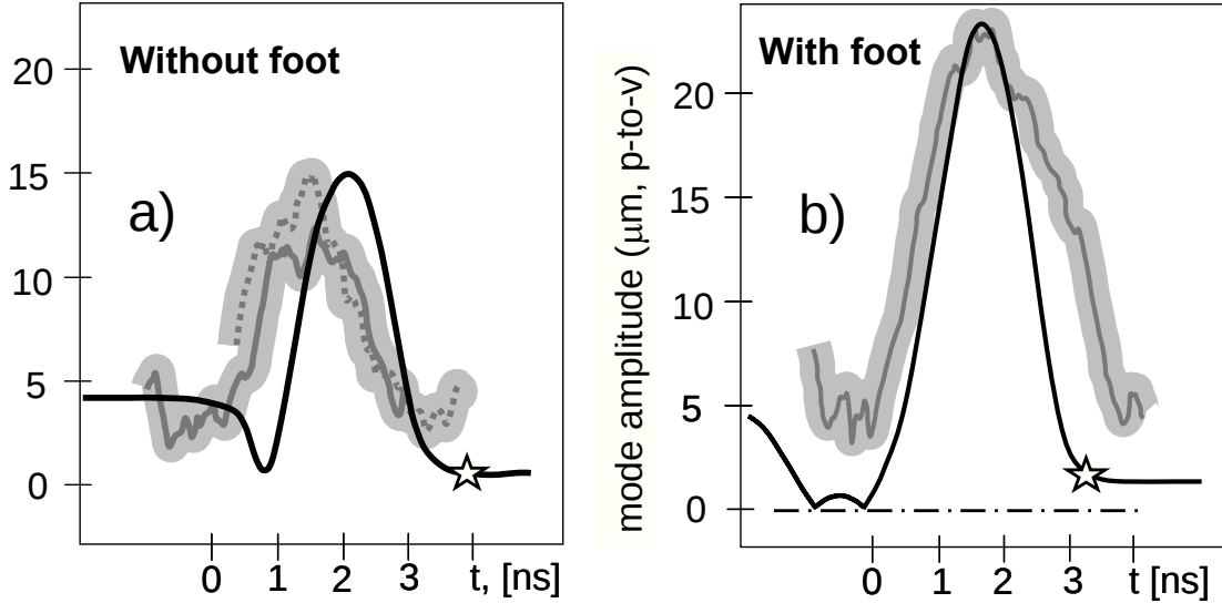
Figure 3. Simulated (black) and measured (gray lines) amplitudes of the dominant Fourier mode for a target irradiated from the plastic side by Nike pulses without (a) and with foot (b). Stars indicate the onset of acceleration. Gray solid and dashed lineouts represent two shots taken consequently in order to cover whole laser pulse without foot. The thickness of the shaded area
