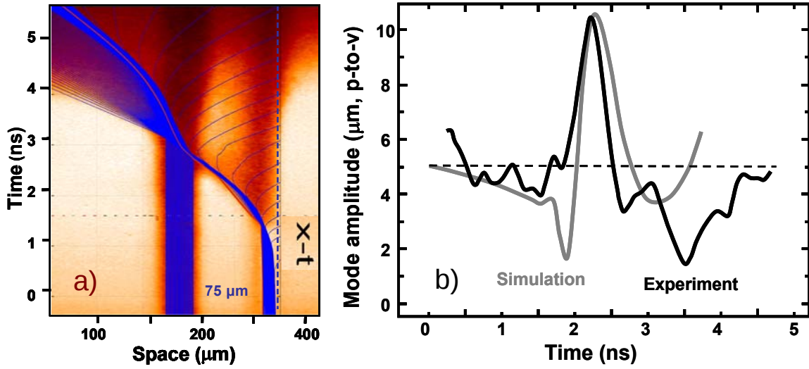
Figure 6. (a) Streak record of the side-lighted double-foil target with rippled front side of the rear foil. Blue lines are x - t trajectories of plasma particles from 1-D simulations. (b) Amplitude of the dominant Fourier mode vs. time for the 30 \mu\text{m} wavelength: experiment (black) and 2-D simulation (gray).
