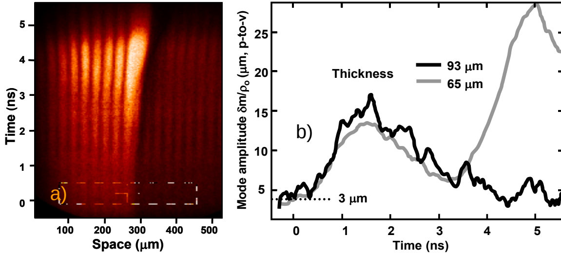
Figure 4. (a) Streak record of the stepped target rippled on the front side. (b) Amplitudes of the dominant Fourier mode vs. time for a 93 \text{ }\mu\text{m} (black) and 65 \text{ }\mu\text{m} thick (gray) parts of the target; horizontal dotted line shows the initial peak-to-valley amplitude.
