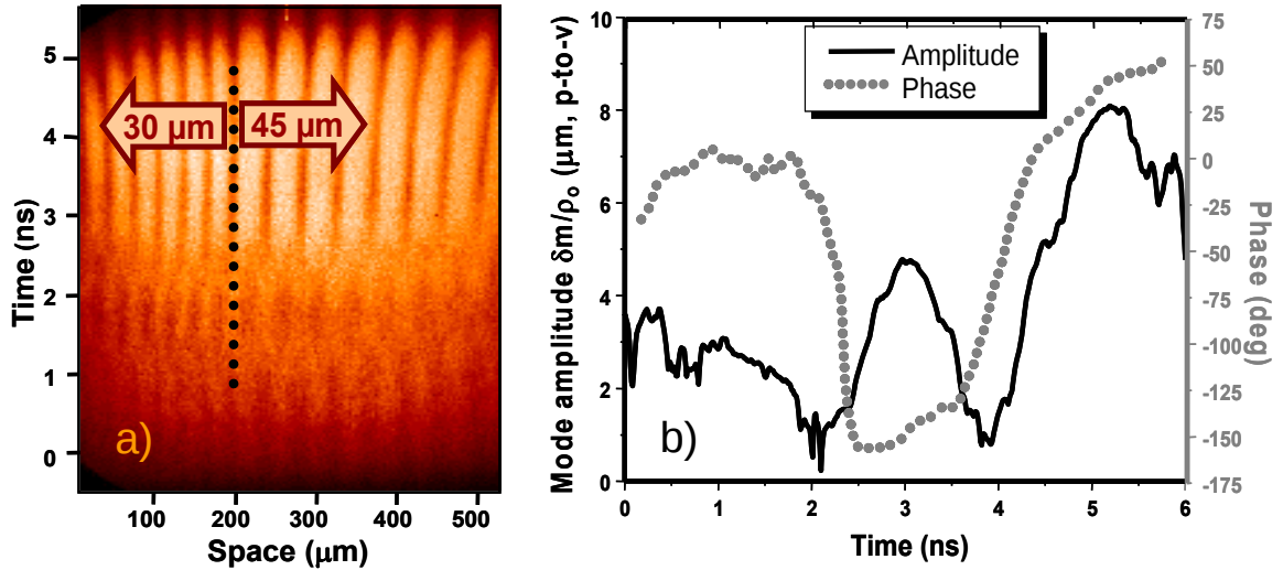
Figure 5. (a) Streak record of a target rippled on the rear side with two wavelengths: 30 μm and 45 μm. (b) Amplitude (black) and phase (gray) of the dominant Fourier mode vs. time for the 45 μm wavelength.
