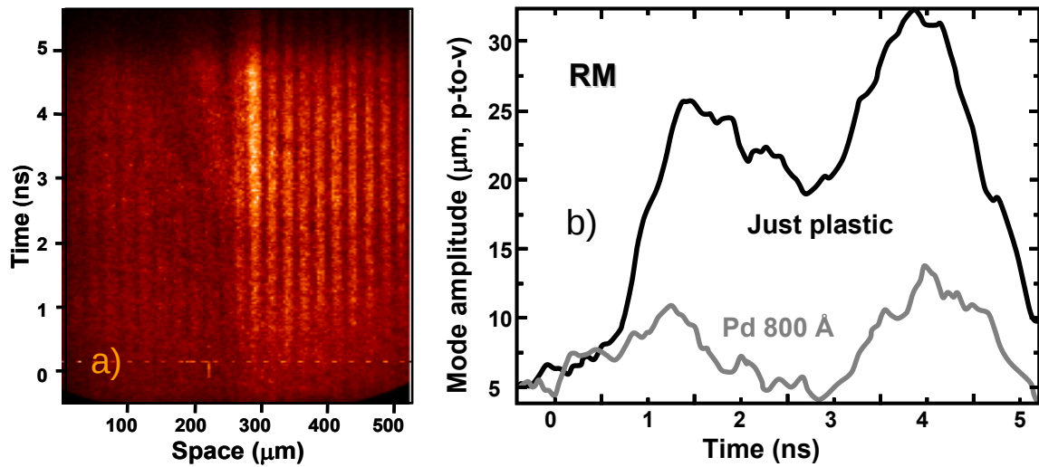
Figure 9. (a) Streak record of the half-coated target rippled on the front side. (b) Amplitude of the dominant Fourier mode vs. time for the uncoated (black) and coated (gray) parts of the target.
