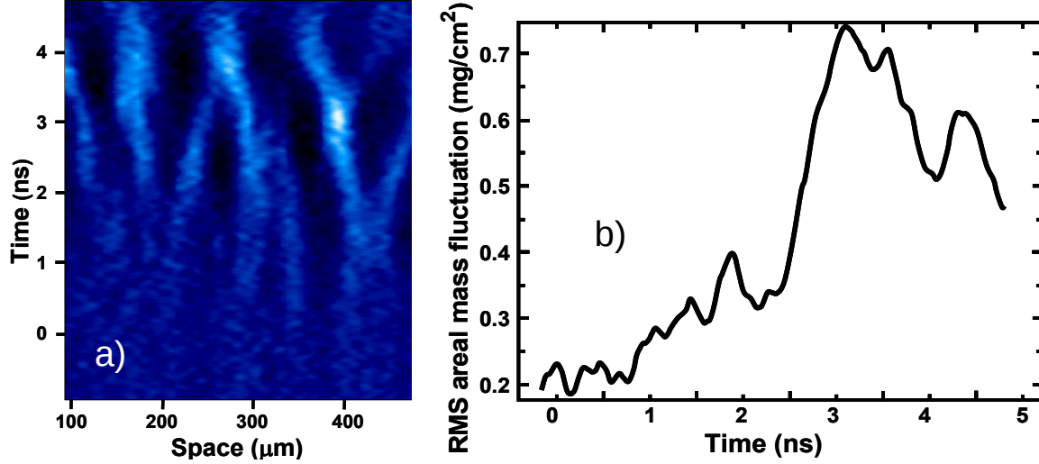
Figure 8. Laser imprint on cryogenic hydrogen-wicked foam: (a) streak image; (b) time history of the rms areal mass fluctuation.
