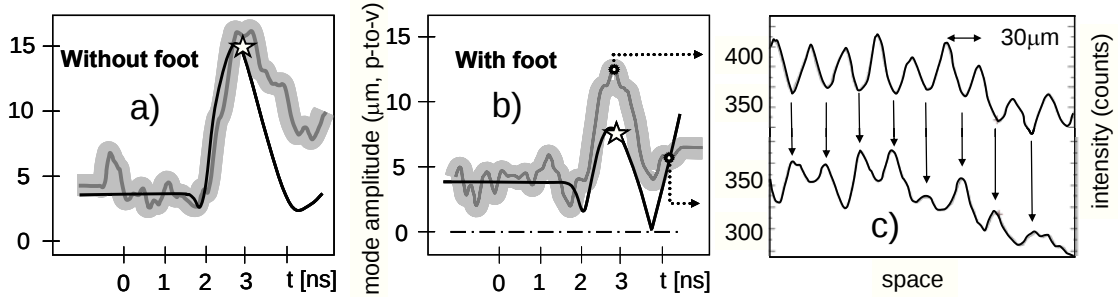
Figure 2. Simulated (black) and measured (gray lines) amplitudes of the dominant Fourier mode for a target irradiated from the foam side by Nike pulses without (a) and with foot (b). Stars in (a), (b) indicate the onset of acceleration. (c) Lineouts of the streak records at 3 and 4 ns showing a phase reversal of areal mass modulation. The thickness of the shaded area approximately corresponds to the experimental uncertainty of the Fourier amplitude measurement near zero.
