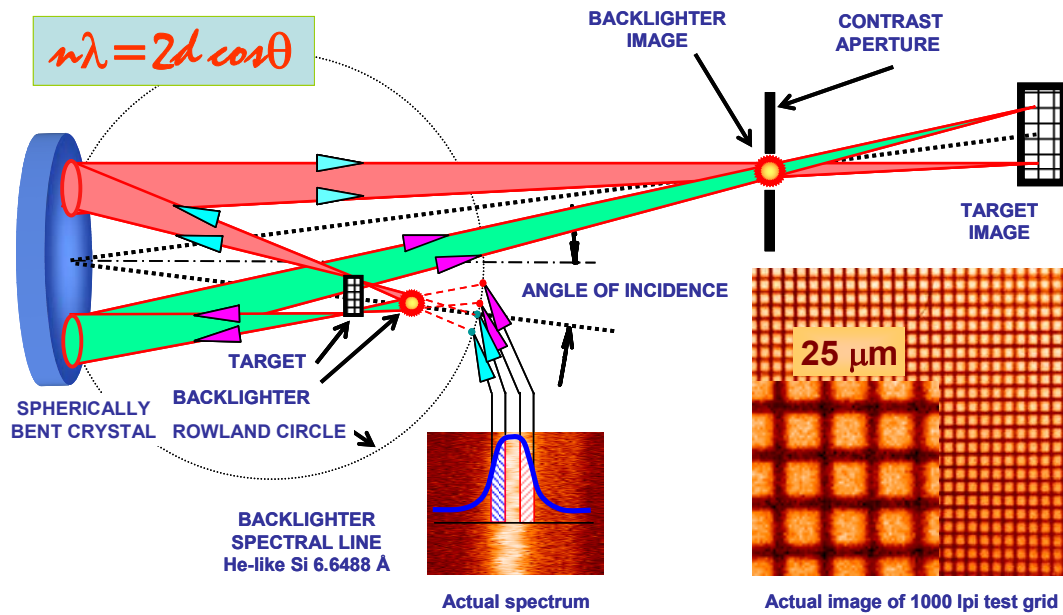
Figure 1. The general scheme of the monochromatic x-ray imaging diagnostics fielded on Nike laser. Also shown: the shape of a Si backlighter spectral line and test images obtained on x-ray film (magnified in the inset).
